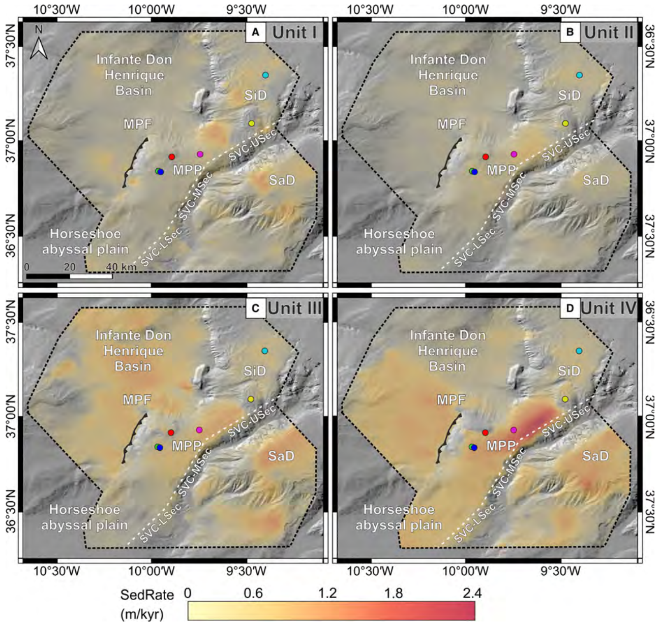
Fig. 6. Decompacted sedimentation rate maps. (A) Unit I; (B) Unit II; (C) Unit III; (D) Unit IV. MPF – Marquês de Pombal Fault; MPP – Marquês de Pombal Plateau; SaD – Sagres Drift; SiD – Sines Drift; SVC – LSec: São Vicente Canyon lower section; SVC – MSec: São Vicente Canyon middle section; SVC – USec: São Vicente Canyon upper section; coloured dots indicate the location of IODP Site U1391 and gravity cores (see Fig. 5 caption for key to colors).
