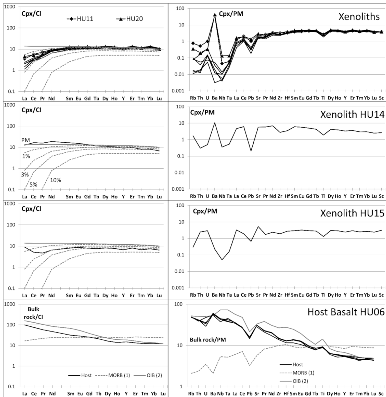
Figure 6. REE and trace elements spiderdiagrams of clinopyroxenes from Huanul mantle xenoliths and host basalt (sample HU06 from Bertotto et al. [41]). REE patterns are normalized to Chondrite-I values (CI) of Lyubetskaya and Korenaga [47]. Spiderdiagrams are normalized to the Primate Mantle (PM) values of McDonough and Sun [48]. The pattern of a primitive mantle-clinopyroxene (solid grey line) of Sun and McDonough [49] and patterns (dotted gray lines) after 1, 3, 5, and 10% of depletion by partial nonmodal melting are also shown. Pattern of MORB [50] and OIB [49] are reported for comparison.
