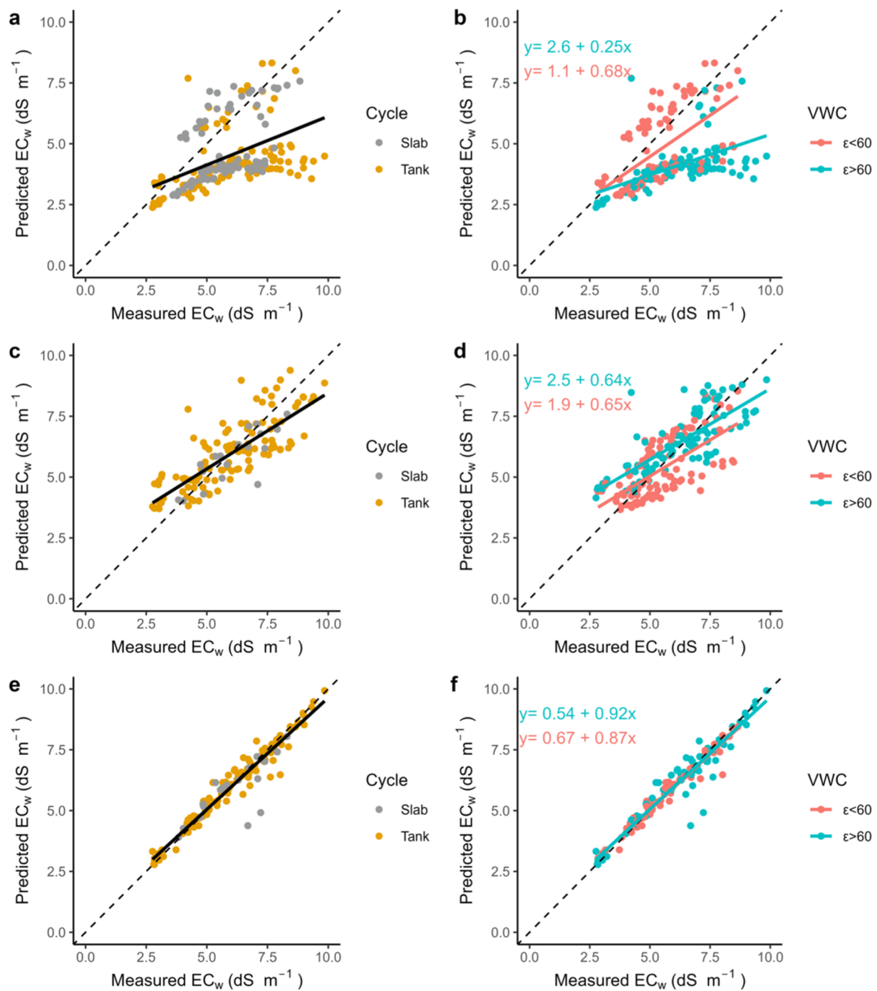
Fig. 5. Comparison between the predicted and the measured pore-water electrical conductivity ( EC_w ) values ( dS\ m^{-1} ) using different models and the “Test” dataset. The linear regression plots show predicted and measured values in the slabs (grey dots) and the tanks (brown dots) using: Hilhorst equation (a), GAM (c), and XGBoost (e). The interactions using two levels of \epsilon_w ( <60 in red and >60 in blue) are shown for: Hilhorst equation (b), GAM (d), and XGBoost (f). The equations are reported in Table 1. (For interpretation of the references to color in this figure legend, the reader is referred to the web version of this article.)
