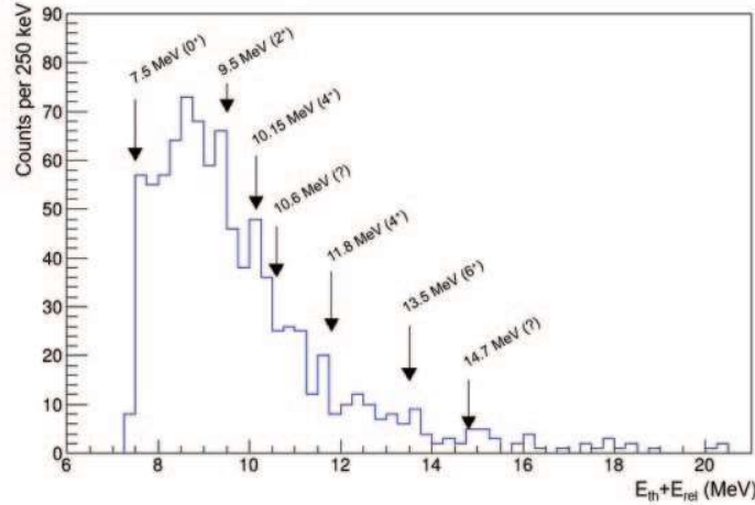
Fig. 2. ^{10}\text{Be} relative energy spectrum reconstructed for the ^4\text{He} + ^6\text{He} decay channel. Positions of various peaks known in literature are marked. In the brackets the J^\pi spin parity is shown.
