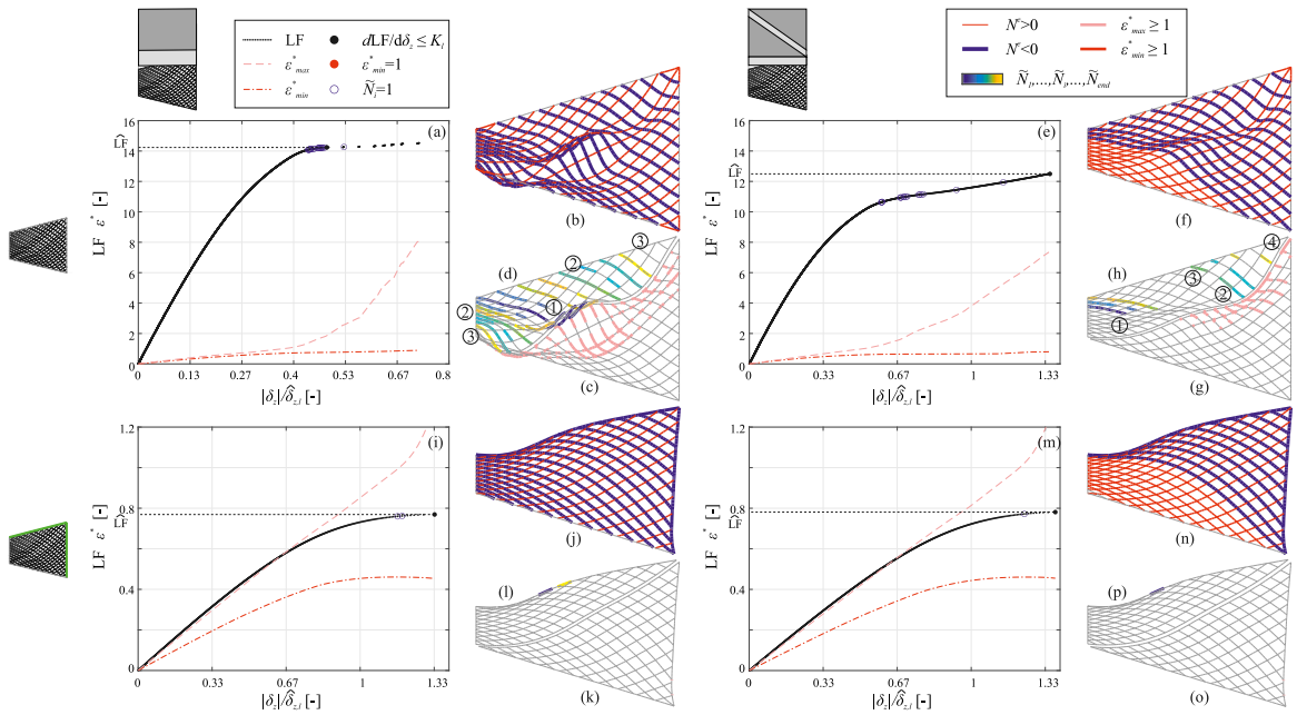
Fig. 13. Hyperbolic paraboloid structural performance: assessment of \widehat{LF} , \epsilon_{max}^* and \epsilon_{min}^* curves (a,e,i,m); members under tension and compression (b,f,j,n); yielded FE for which \epsilon_{max}^* \geq 1 and \epsilon_{min}^* \geq 1 (c,g,k,o); and members subjected to progressive buckling (d,h,l,p) over gridshell deformed shape at ULs.
