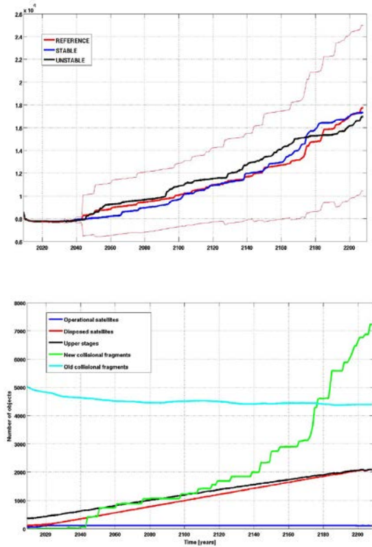
Fig. 1. Top panel: Effective number of objects between 15000 and 35000 km, larger than 5 cm in the three scenarios: Reference (thick red line), Stable (blue line) and Unstable (black line). The thin red lines show the \pm 1 sigma of the MC averaging in the Reference case. Bottom panel: Effective number of objects between 15000 and 35000 km, larger than 5 cm divided by type: operational satellites (blue), disposed satellites (red), upper stages (black), old collisional fragments (cyan) and new collisional fragments (green).
