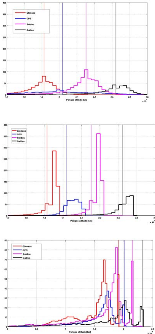
Figure 2. Perigee altitude distribution, in the year 2209, of the disposed satellites in the Reference (top panel), Stable (middle) and unstable (bottom) scenarios. The thin vertical lines mark the altitude of the four GNSSs operational orbits.
