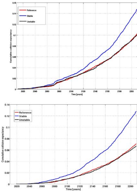
Figure 3. Top panel: cumulative collision expectancy for objects belonging to the GNSSs (both operational and disposed) in the three main scenarios: Reference (red), Stable (blue) and Unstable (black). Bottom panel: cumulative collision expectancy for non-operational objects belonging to the GNSSs against every other non-controlled object (i.e., other GNSSs non-operational, upper stages, fragments, MRO,...). See text for details.
