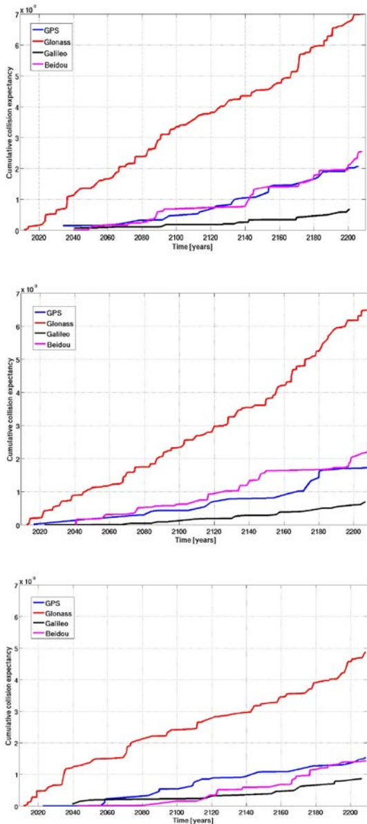
Figure 4. Cumulative collision expectancy for operational satellites belonging to the four GNSSs in the Reference (Top panel), Stable (middle panel) and Unstable (bottom panel) scenarios. The red line refers to Glonass, the blue line to GPS, the magenta line to Beidou and the black line to Galileo
