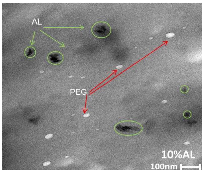
Figure S1: TEM micrograph of TPZ filled with 10wt% of AL
