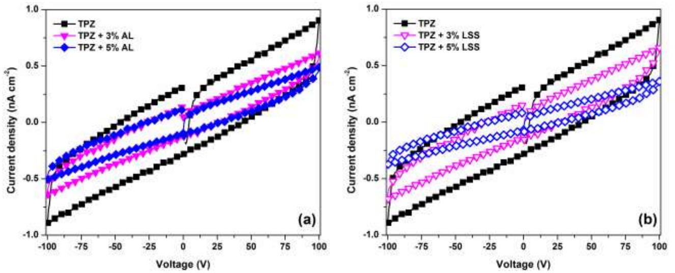
Figure S2: Current density-voltage characteristics of aged TPZ and TPZ-based bio-nanocomposites containing 3 and 5 wt% of (a) AL and (b) LSS
