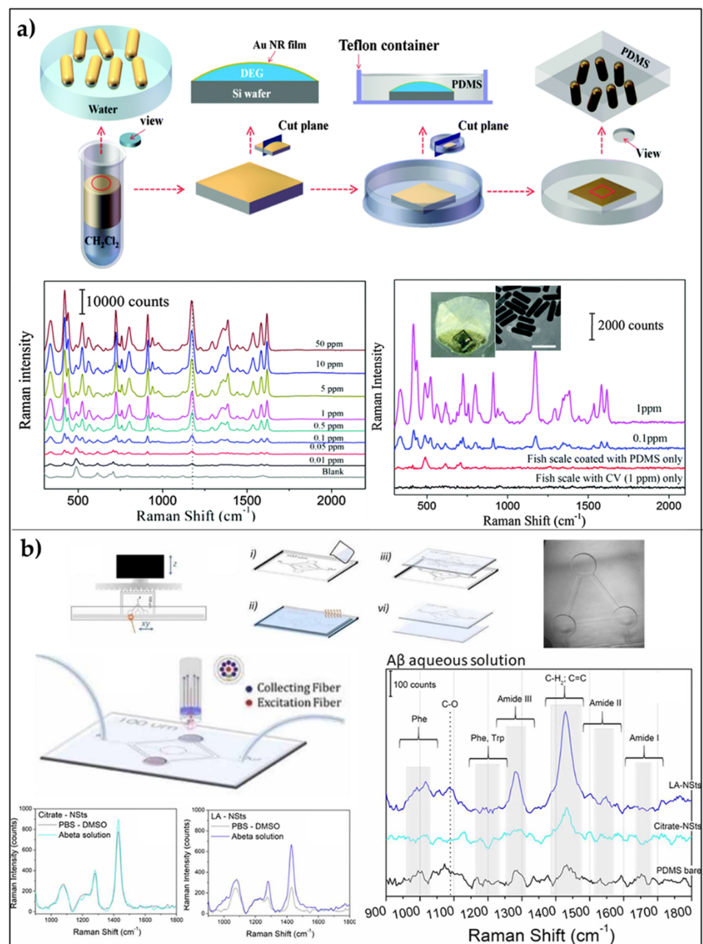
Figure 5. SERS platforms based on transparent polymers: (a) AuNRs/PDMS platform: schematic illustration of the preparation of AuNRs/PDMS substrate, SERS spectra of aqueous CV at various concentration, and SERS spectra of CV acquired by applying the nanocomposite film on the fish scale and then illuminating from the backside with a 785 nm laser. Adapted with permission from [101]. Copyright (2017) American Chemical Society. (b) AuNSs/PDMS microfluidic channel for SERS: Schematic illustration of the fabrication process of depicting the final device coupled with the Raman fiber probe; Raman spectra of \beta -42-peptide against buffer solution for Citrate-AuNSs substrates, and LA-AuNSs-PDMS; finally, a comparison of the background-subtracted Raman ‘fingerprint’ spectral region of \beta -42-peptide between bare PDMS, Citrate-AuNSs, LA-AuNSs substrates. Adapted with permission from [50]. Copyright (2020), IOP Publishing Ltd.
