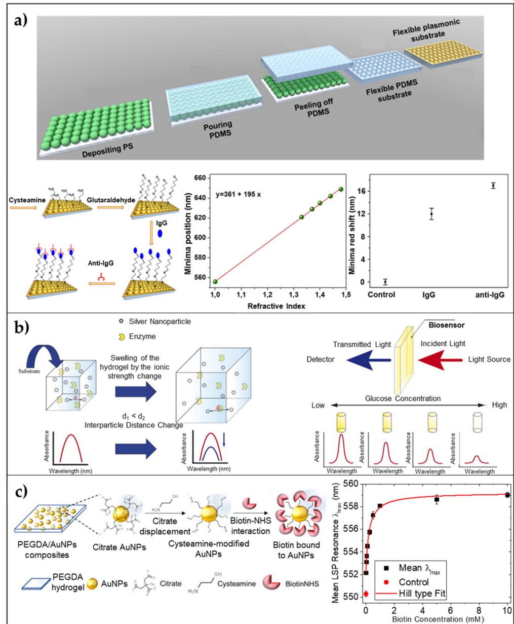
Figure 3. 3D arrays of AuNPs on/embedded in flexible substrates/matrices. (a) 3D Nanocups on PDMS: Schematic illustration of the fabrication steps of the flexible 3D Au nanocups platform; sensitivity measurements leading to a value of 195 nm/RIU; and reflectance response after human IgG immobilization and specific anti-human IgG detection Adapted from ref. [80] Copyright (2017) with permission from Springer Nature. (b) Stimuli-responsive hydrogel embedding AgNPs: Schematic illustration of detection principle of LSPR-based optical enzyme biosensor. Reproduced from Ref. [81] Copyright (2008), with permission from Elsevier. (c) PEGDA hydrogel nanocomposite embedding AuNPs: Schematics of the functionalization procedure involving citrate displacement with a cysteamine modification of AuNPs and the subsequent sulfo-NHS biotin grafting on the available amino groups of cysteamine within the nanocomposite, and LSPR \lambda_{max} (black squares) as a function of the biotin concentration (from 25 \mu M to 10 mM). Adapted from [17] Copyright (2021), with permission from AIP Publishing.
