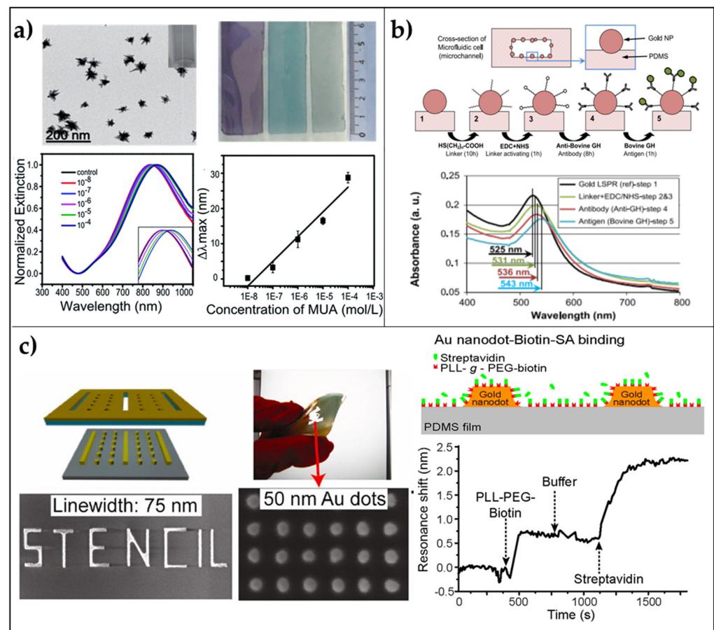
Figure 2. 2D arrays of AuNPs on PDMS flexible substrates. (a) Immobilization of AuNSs on PDMS: TEM images of gold nanostars (scale bar 200 nm); macroscopic morphology of PDMS/AuNSs platforms; extinction spectra of a PDMS/AuNSs film immersed in different concentrations of MUA in ethanol; LSPR shift versus MUA concentration. Reproduced from [71] with permission from Royal Society of Chemistry Pub. (b) In situ growth of AuNPs in a microfluidic chamber: Biosensing experiments performed by using the annealed microfluidic biosensor (400–2 cells) prepared from 2% aqueous solution of the gold precursor (48 h); cross-section of a microchannel and AuNPs in the channel; four steps of the biosensing protocol; a legend of the schematics; Au-LSPR corresponding to the four sensing steps, and LSPR band shift corresponding to different Ag concentrations. Reproduced from [72] Copyright (2013), with permission from Elsevier. (c) Patterning via Nanostencil Lithography: Schematics of biosensing experiments with nanodots on PDMS. Au nanodots and PDMS are biotin-functionalized, and then streptavidin binds to biotin. LSPR shift of an array of W = 75 nm and S = 50 nm Au nanodots on PDMS upon the addition of biotinylated molecules and streptavidin. The arrows indicate the addition of biomolecules and buffer rinsing. Adapted from [73]. Copyright (2012) with permission from American Chemical Society.
