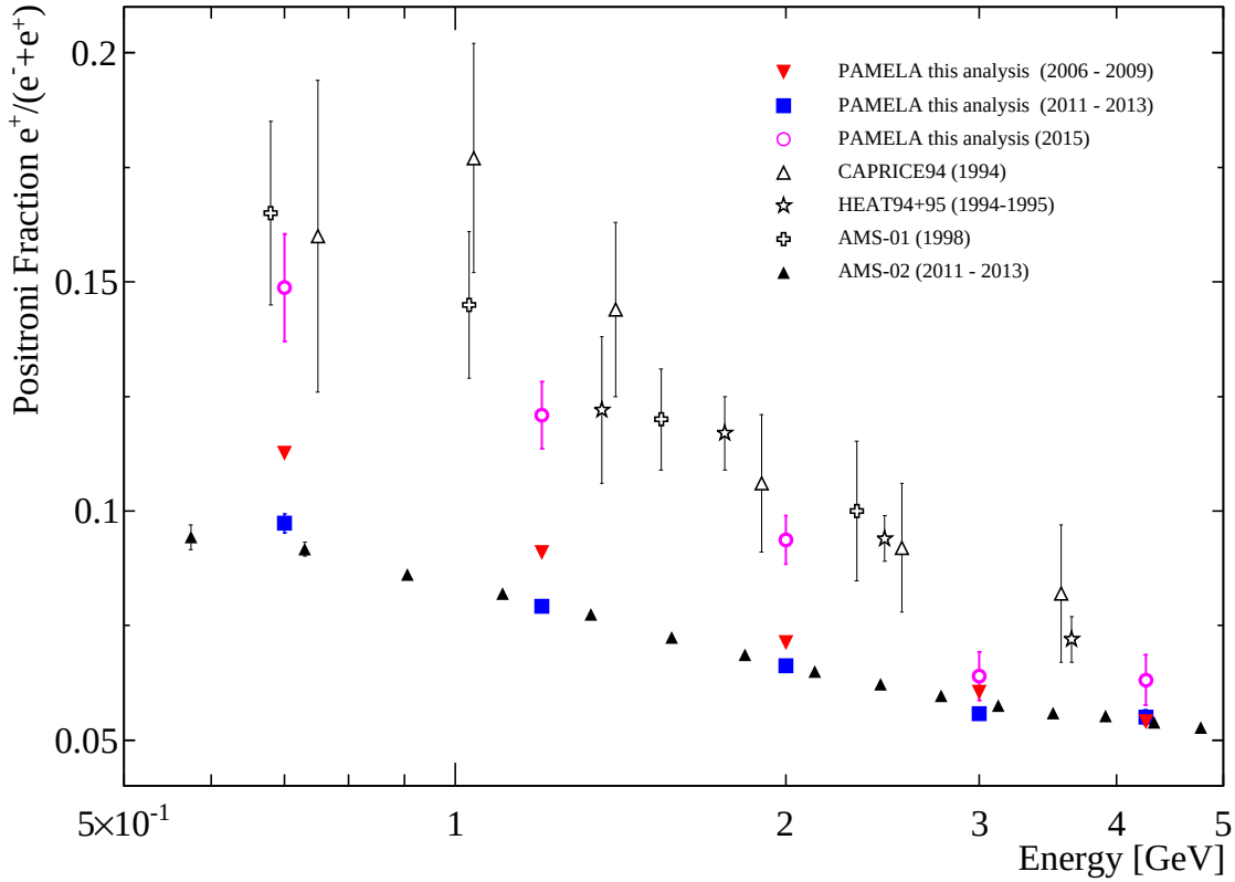
FIG. 2: The positron fraction derived in this work for three time periods: July 2006-December 2009, (solar minimum, as in [5]), May 2011-November 2013 (as AMS-02 results [8]), January-December 2015, along with other recent measurements: HEAT94+95 [15], CAPRICE94 [16], AMS-01 [17], AMS-02 [8]. The results from [15–17] refer to the previous A > 0 solar cycle.
