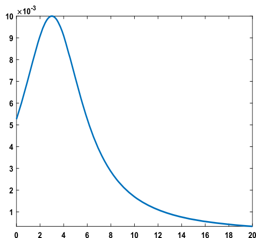
Fig. 2. Example 2: pointwise absolute errors for n = 350 , \theta = 0.2 (left), function f (right).
