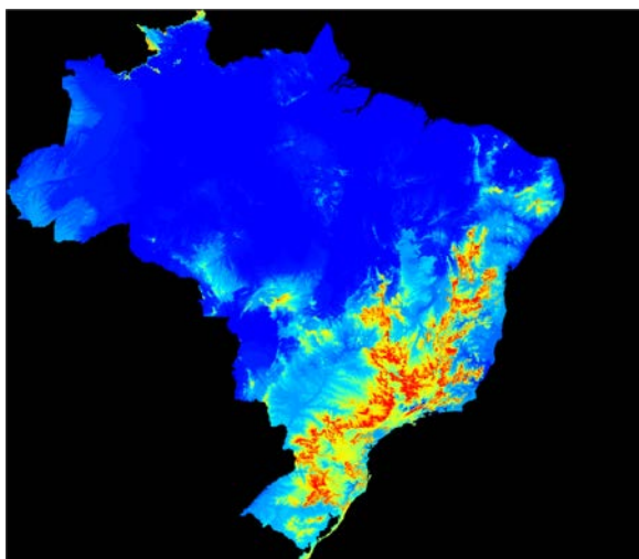
Figure 15 - Potential distribution of Passiflora amethystina obtained with the ENFA algorithm
