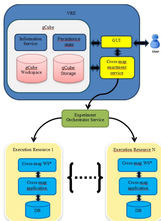
Figure 24 – Improved architecture for UCI
