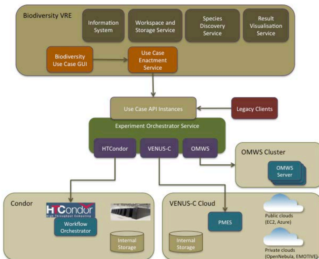
Figure 11 – Implementation of the Use Cases on the EUBrazil OpenBio Infrastructure
