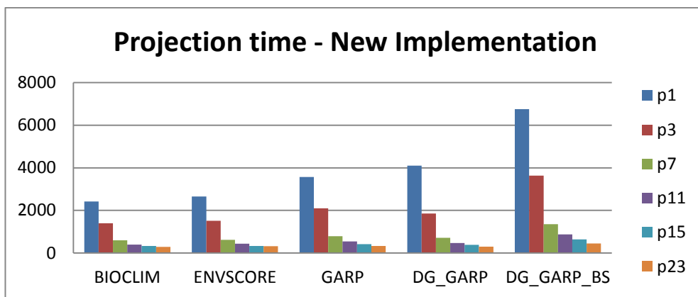
Figure 22 – Execution times (in seconds) obtained by the new parallel version of om_project
