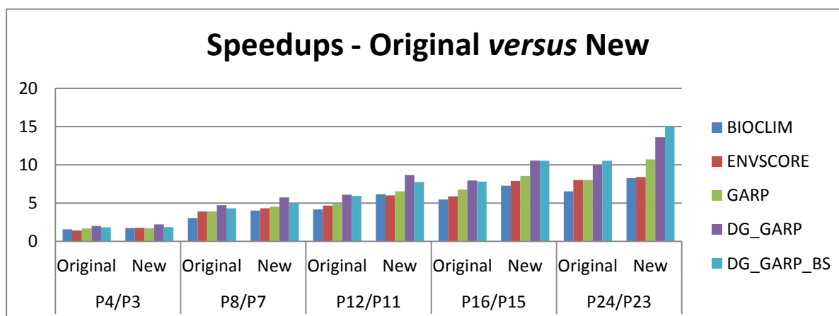
Figure 23 – A comparison of speedups achieved by the parallel versions of om_project
