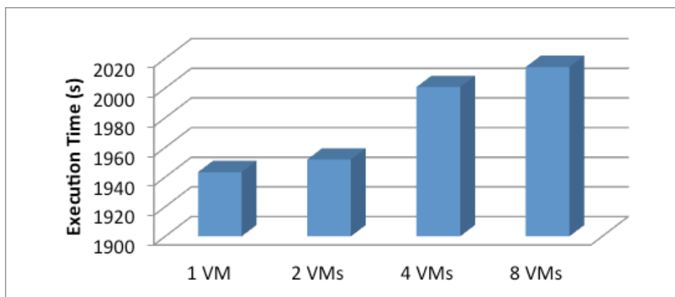
Figure 18 - Average execution times for an increasing number of concurrent VMs
