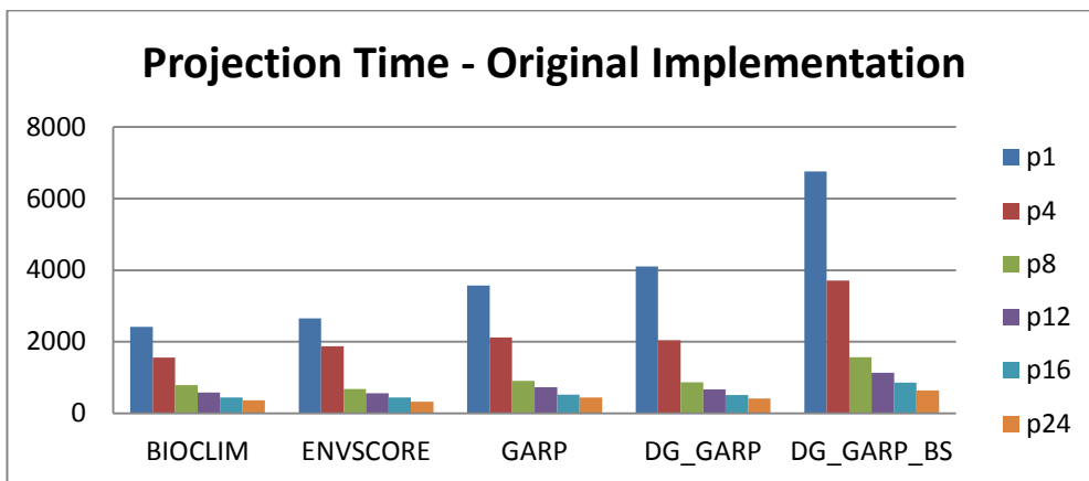
Figure 21 – Execution times (in seconds) obtained by the existing parallel version of om_project
