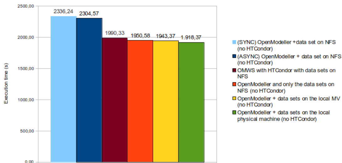
Figure 19 – Average execution time of one instance of OpenModeller with the modelling algorithm ANN
