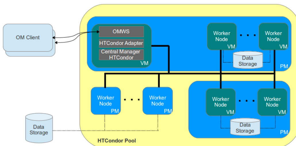
Figure 17 - Current HTCondor Pool Configuration
