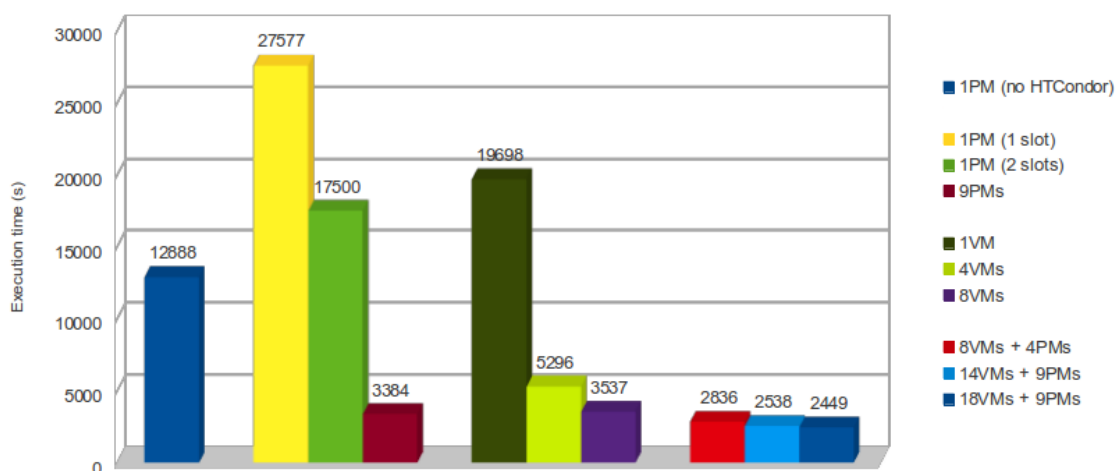
Figure 20 - Average execution time of one instance of openModeller with ANN as the modelling algorithm
