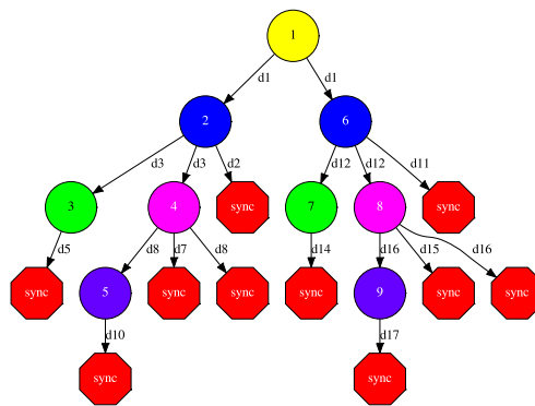
Figure 13 - ENM COMPSs workflow with 1 species and 2 algorithms
