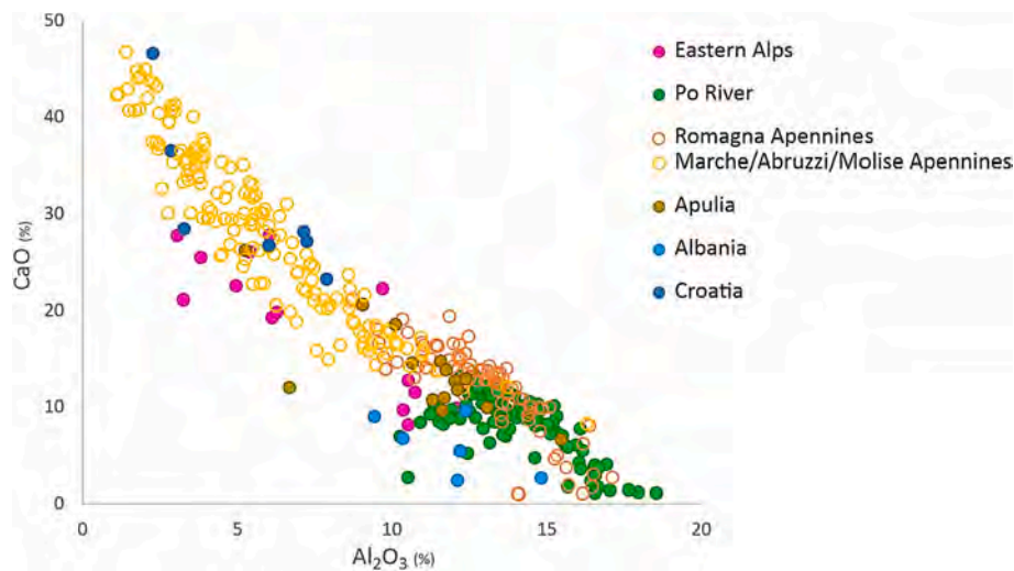
Fig. 5. Scatterplot of CaO versus \text{Al}_2\text{O}_3 from fluvial, deltaic and lacustrine deposits of the Po-Adriatic system. The highest Ca values reflect erosion and transport of detrital calcite from limestone-rich sediment sources (Croatian Dinarides, Marche/Abruzzi Apennines and Eastern Alps - see catchment geology in Fig. 1). Albanian samples from Salminen et al. (2005) and Shtiza et al. (2009); Croatian samples from Miko et al. (2003b), Salminen et al. (2005), and Ilijanić et al. (2022).
