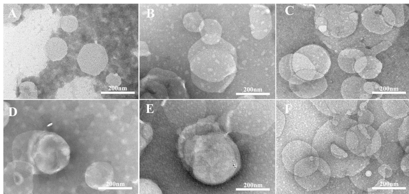
Fig. 2. TEM micrographs of liposomal formulations (negative staining) before (A, B, and C) and after (D, E, and F) nebulization. LipoINH (A and D), LipoINH + Chit (B and E,) and LipoINH + ε-PLL (C and F).
