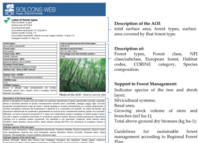
Figure 5. Results from three simulations of the GIFT tool. Three identical areas of interest (AOI) have been generated according to the forest stand information the user was interested to get (canopy cover or growing stock volume). Accordingly, a technical report has been created with information of the AOI. The original information is in Italian (here translated manually in English) since the platform has been designed for Italian forest owner use.
