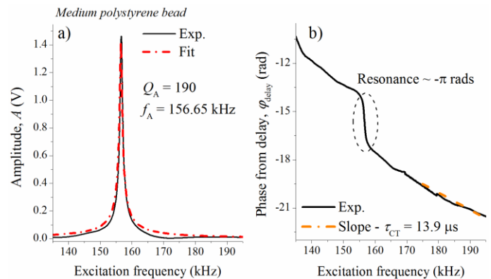
Fig. 3. Experimental amplitude and phase measured in open-loop mode for the cantilever with the medium polystyrene bead attached. a) The damped harmonic oscillator model is fitted (red dashed-dotted line) to the measured amplitude (solid black line) and the parameters are extracted; b) The delay on the propagation of the elastic waves through the holder and cantilever materials is extracted from the slope of the phase spectrum away from the resonance. The resonance occurs at 156.65 kHz, as indicated in Table II.
