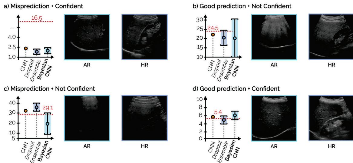
Fig. 5. Comparison of predictions and level of uncertainty for 4 cases with different percentage of FLC. a) Case predicted with low precision and small amount of uncertainty. b) Case predicted with good precision and big amount of uncertainty. c) Case predicted with low precision and big amount of uncertainty. d) Case predicted with good precision and small amount of uncertainty.
