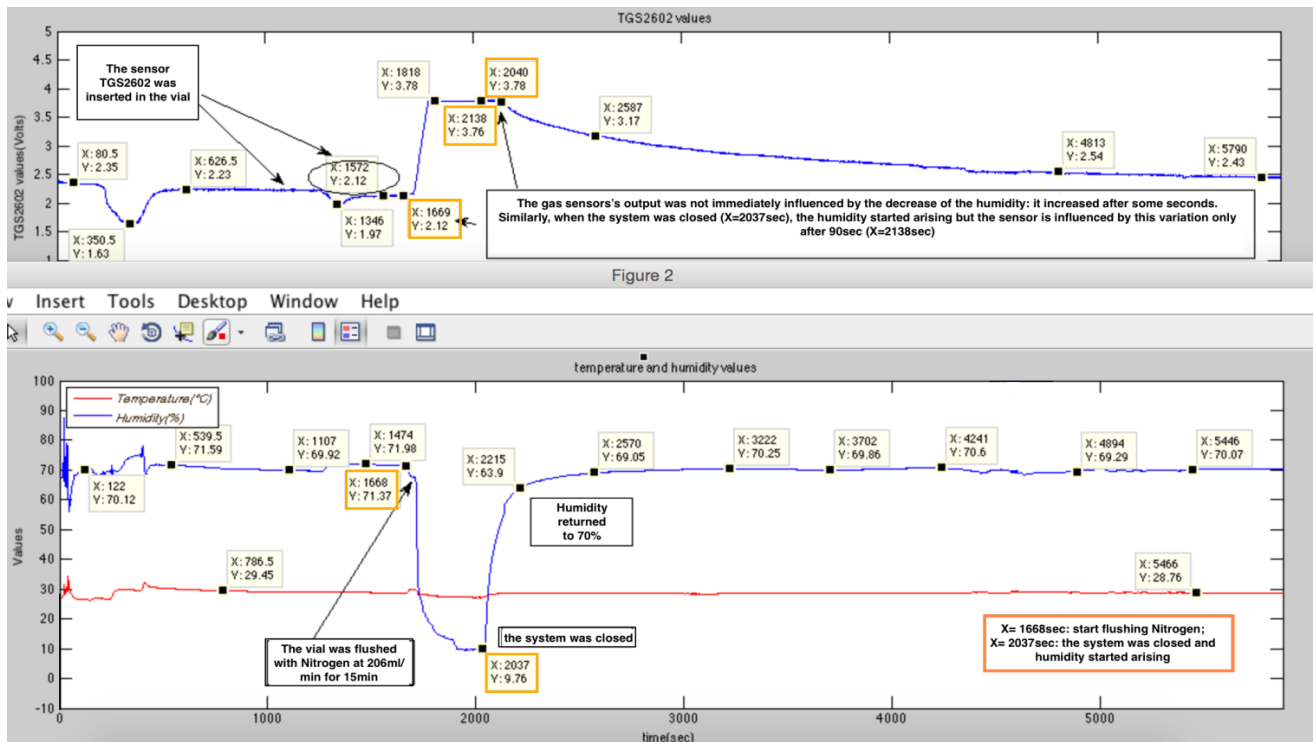
Figure 10 - TGS2602 was inserted into the vial; then the vial was flushed with Nitrogen at 206ml/min for 15min.
