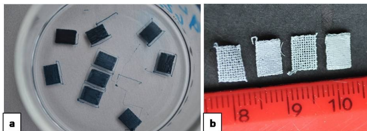
Figure 7 -(a) Wet-spun microstructured membranes. (b) Dried microstructured membrane prototypes; from left to right: PHBHHx/PAni- d_F 0.2 N_L 4, PHBHHx/PAni- d_F 0.5 N_L 4, PHBHHx/PAni- d_F 0.5 N_L 8 and PHBHHx/PAni- d_F 0.2 N_L 8.
