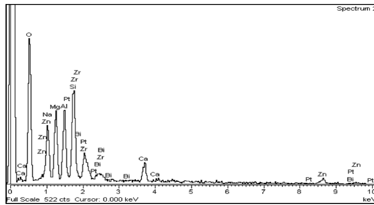
Figure 15- Chemical composition of the metal oxide structure. The results show that the prevalent compound is the ZnO 2 , with several doping atoms, such as Zr, Si, and Bi.
