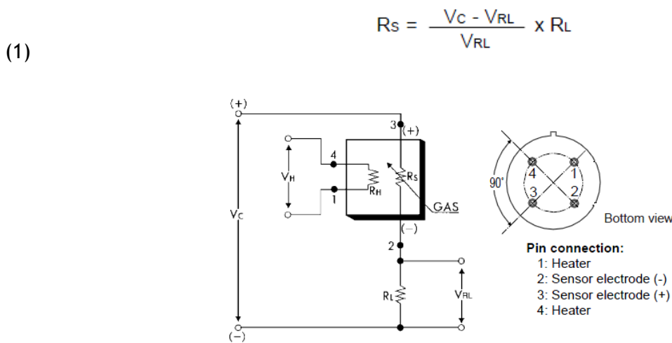
Figure 1- The inner electrical circuit
