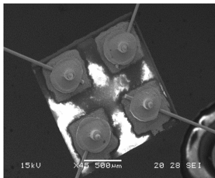
Figure 12- SEM overview of the hybrid sensor metal oxide/PANi
