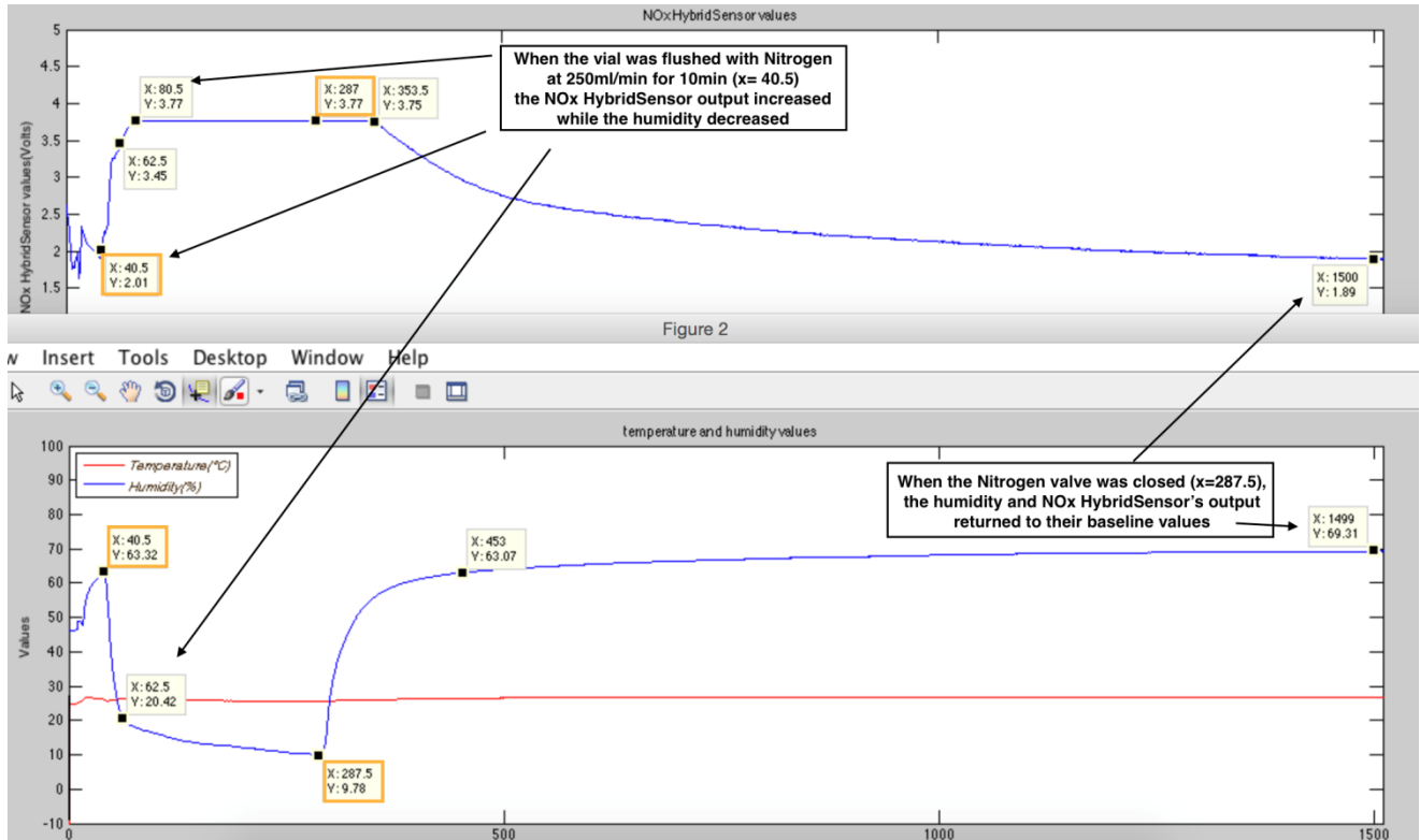
Figure 19- Flush with Nitrogen at 250ml/min for 10min. When the Nitrogen valve was closed, both the sensors returned to their baseline value, that is 1.89V @69.31% humidity for NOx Hybrid Sensor.
