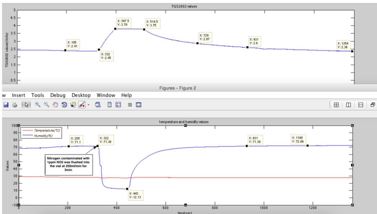
Figure 11- We demonstrated that TGS2602 is not sensitive to Nitrogen Oxide
