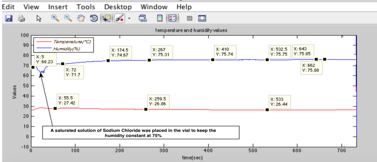
Figure 9- The humidity in the vial was kept constant at 75% by means of a saturated solution of Sodium Chloride
