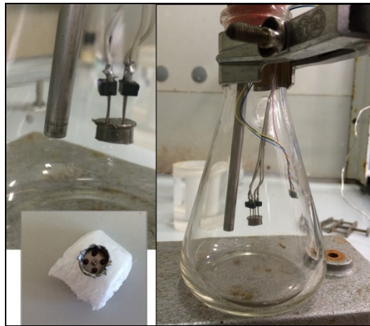
Figure 18- Test set-up for NOx Hybrid-Sensor. Here the TGS2602 “cut” in order to settle PANi sol-gel nanofilm on its sensing element.
