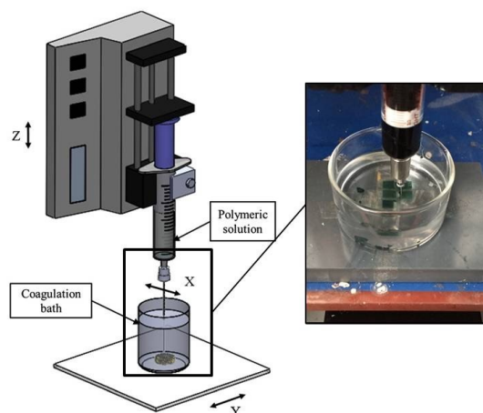
Figure 6 -Schematics of the computer-aided wet-spinning (CAWS) system employed for the preparation of PHBHHx/PAni blend microstructured membranes.
