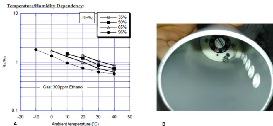
Figure 2 (A) An example of the effects of temperature and humidity on gas sensors' sensitivity (TGS2602 in this case). (B) Sensirion SHT11 temperature sensor inside the store chamber.
