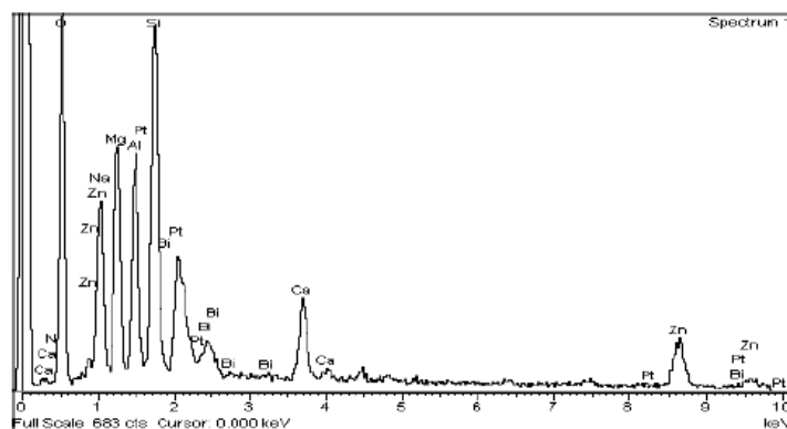
Figure 17- Since carbon atoms form the initial high peak, the PANi structure’s chemical composition is evidenced by the presence of N atoms, between Ca and O atoms.
