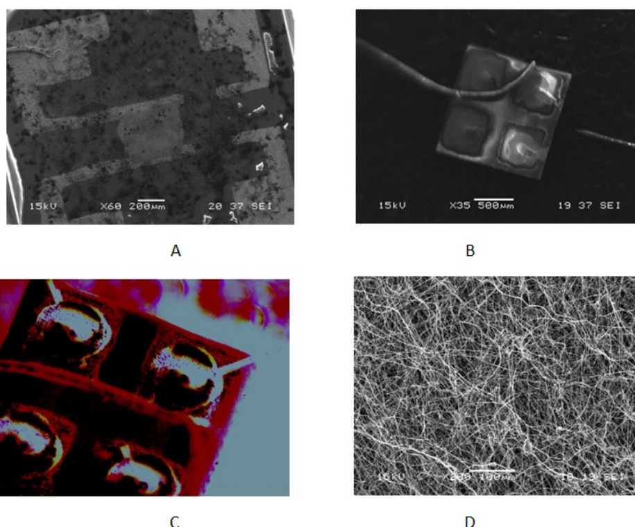
Figure 5- Surfaces of hybrid sensors (metal-oxide/PANi) as observed using a SEM. A, PANi nanoislands produced with the dip-coating technique; B and C single wet-spun microfiber PANi; D, electrospun nanofibers.
