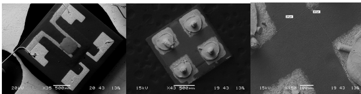
Figure 4- Example of sensing surfaces for two different FIGARO sensors. The images were recorded with a Scanning Electron Microscope
