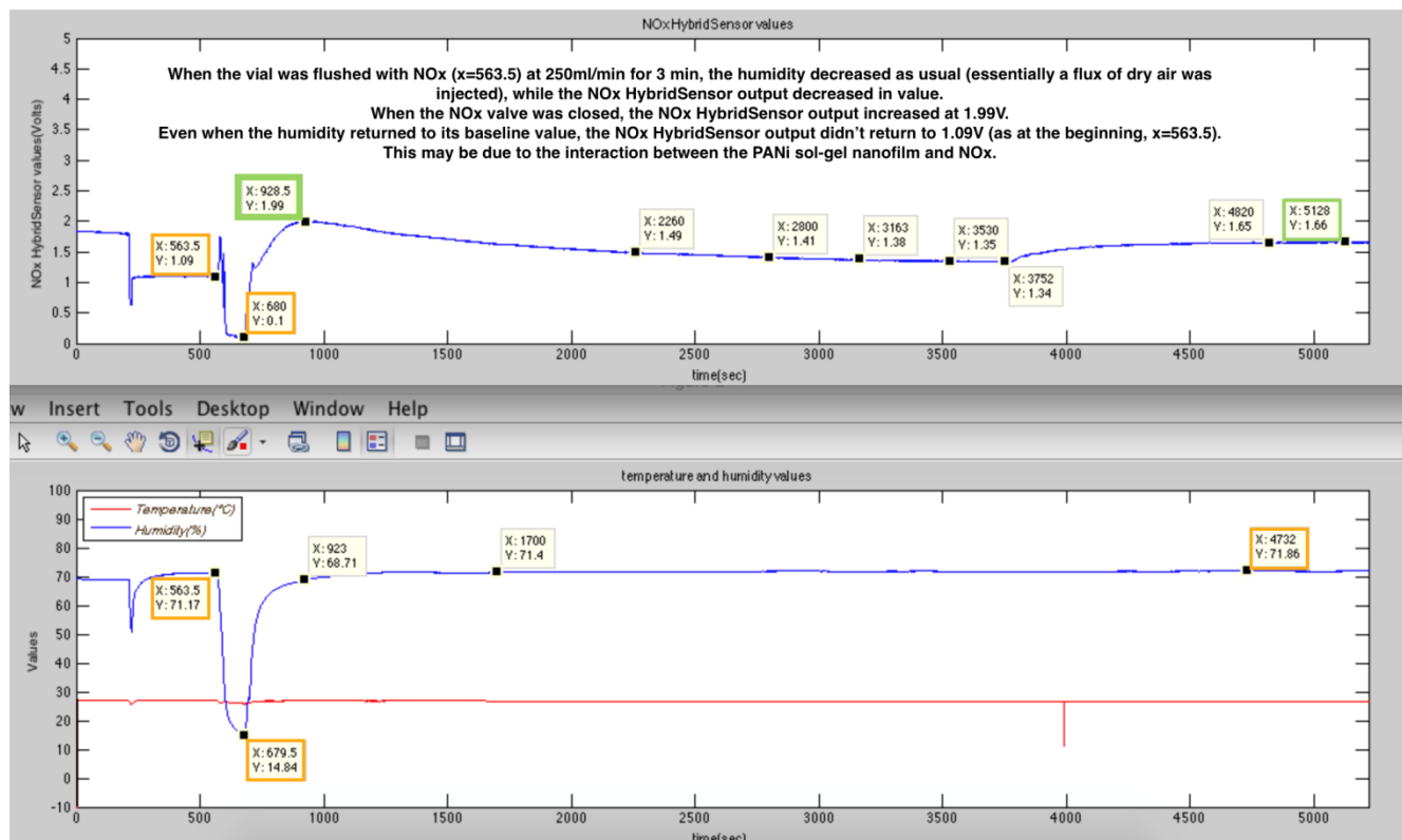
Figure 20- NO x Hybrid Sensor's sensitivity to Nitrogen Oxide.
