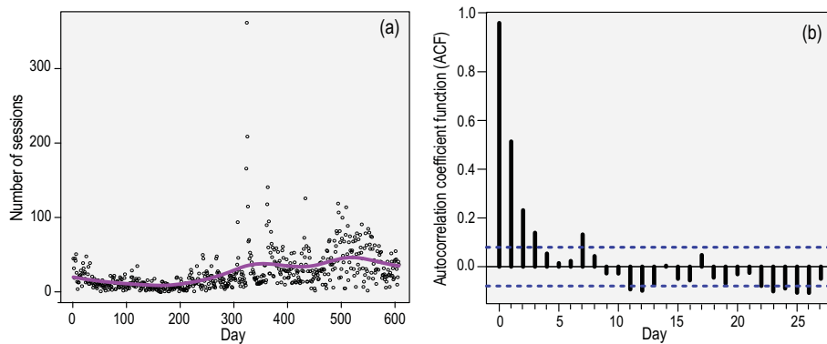
Figure 5. (a) Plot shows the original data (points) and the line (violet line) describing its trend. (b) Chart shows autocorrelation coefficient function (ACF) calculated using the time series of the number of sessions of the POLARIS website.
