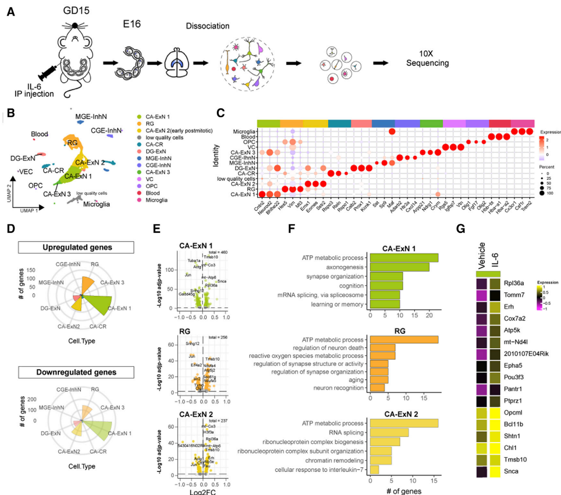
Figure 2. Single-cell sequencing of embryonic brains exposed to IL-6 reveals a deep transcriptional rearrangement in neuronal populations and engagement of key biological processes in synaptogenesis
