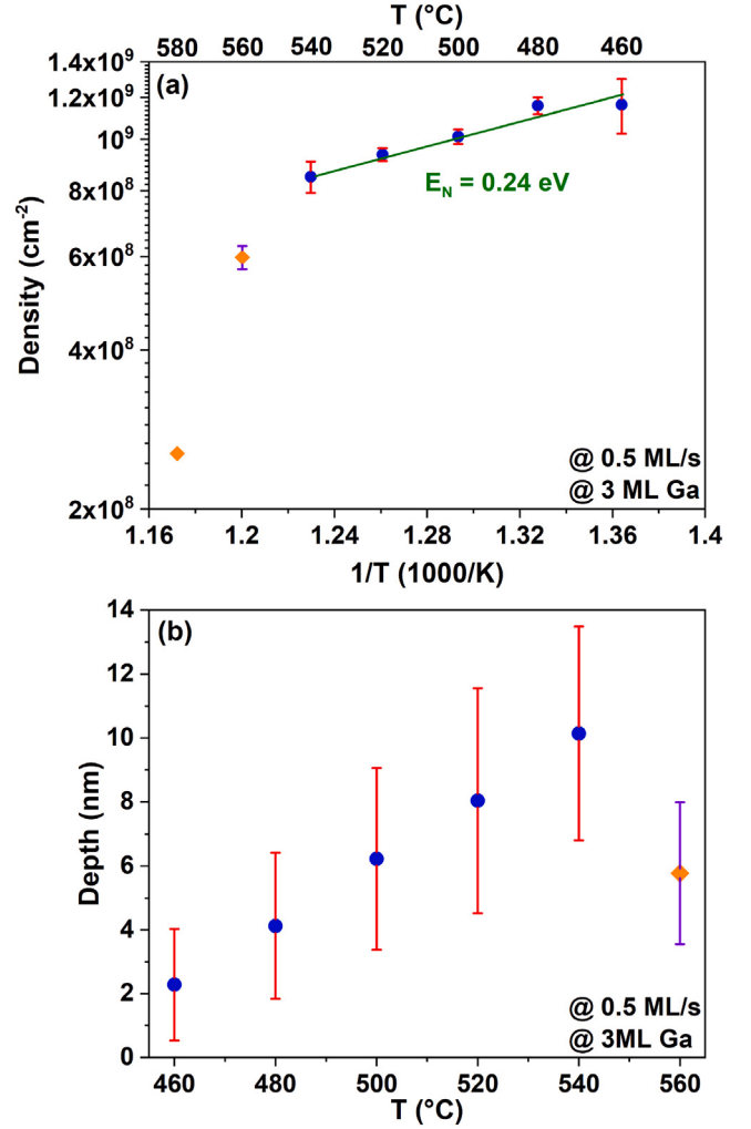
Fig. 3. T series : The temperature dependencies of (a) the nanopit density and (b) the nanopit depth. F_{Ga} and \Theta_{Ga} during the fabrication of the sample series are 0.5 ML/s and 3 ML, respectively. Samples T6 and T7 affected by the indium desorption are highlighted by orange points with violet error bars.
