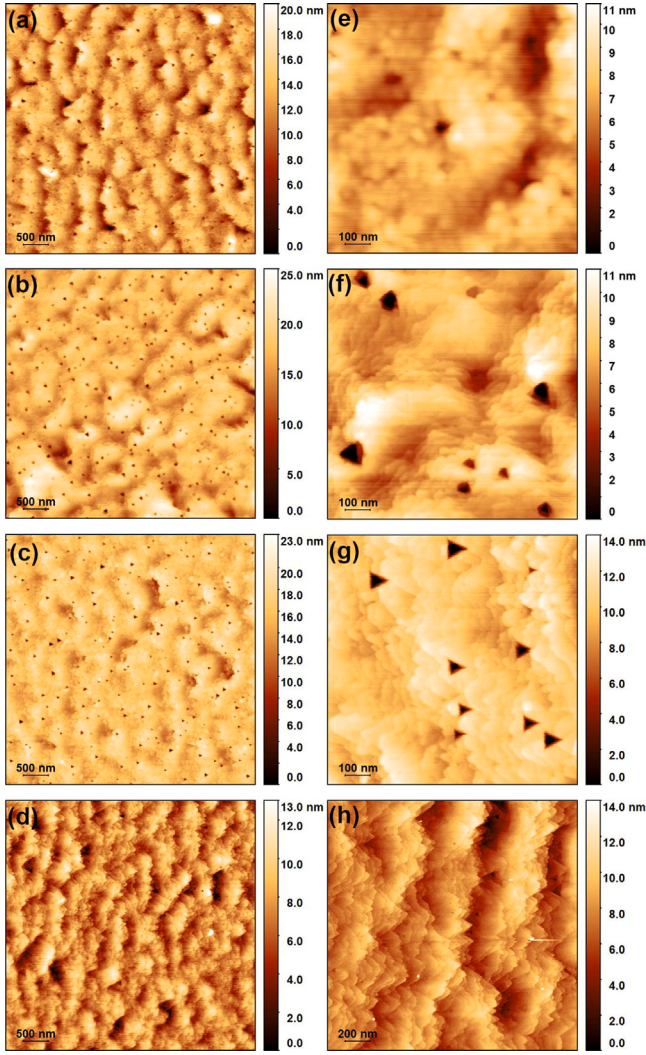
Fig. 2. T series : AFM topography images of samples T1 — (a) 5 \times 5 \mu\text{m}^2 , (e) 1 \times 1 \mu\text{m}^2 ; T3 — (b) 5 \times 5 \mu\text{m}^2 , (f) 1 \times 1 \mu\text{m}^2 ; T5 — (c) 5 \times 5 \mu\text{m}^2 , (g) 1 \times 1 \mu\text{m}^2 ; and T7 — (d) 5 \times 5 \mu\text{m}^2 , (h) 2 \times 2 \mu\text{m}^2 .
