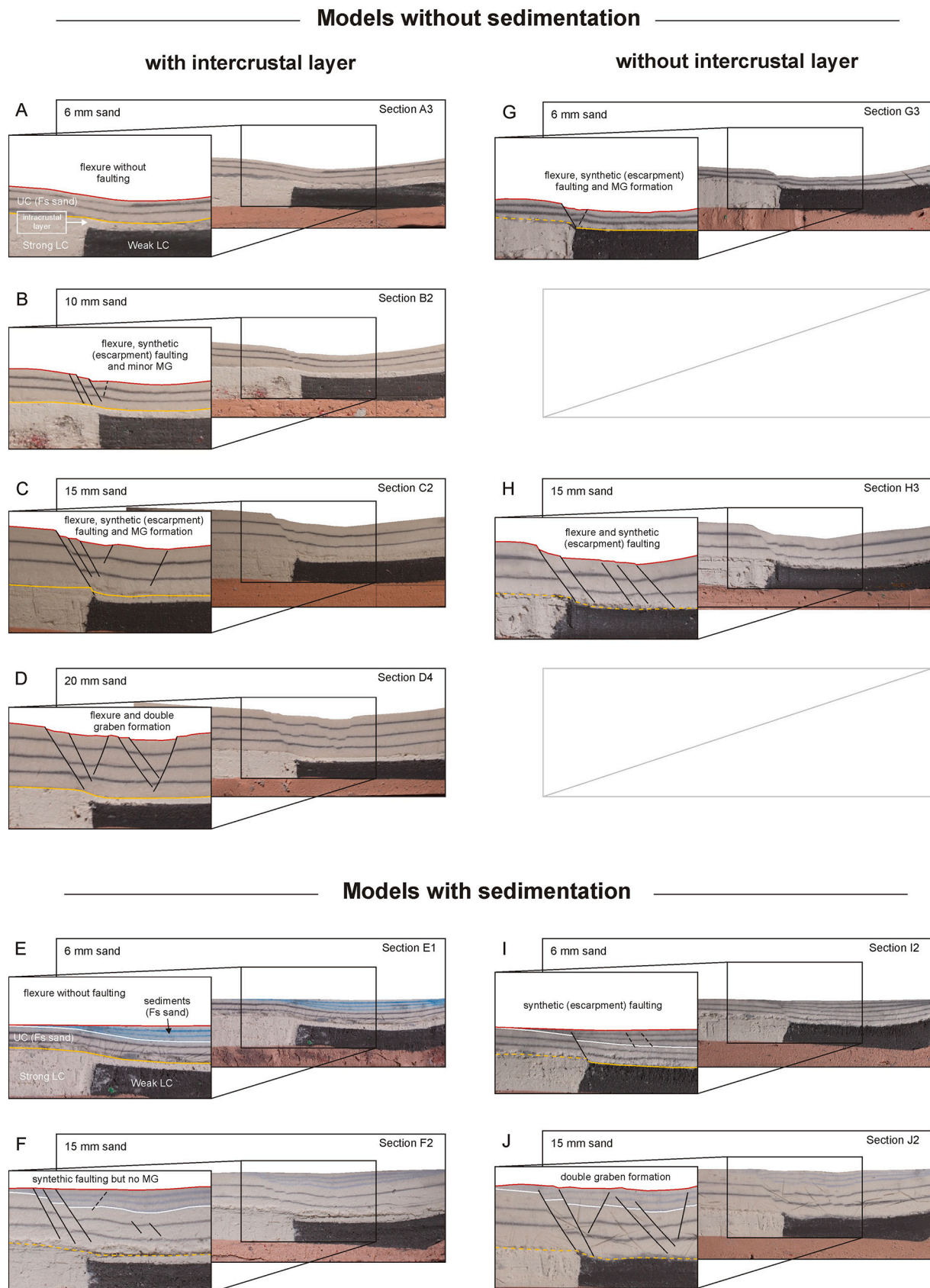
Fig. 4. Cross-section summary of final series 1 model structures as a function of brittle layer thickness, the presence of a thin intra-crustal layer and sedimentation. Insets show our structural interpretation. The strong and weak lower crustal analogues are light grey and black, respectively. LC: lower crust, MG: marginal graben. Section locations are shown in Fig. 3.
