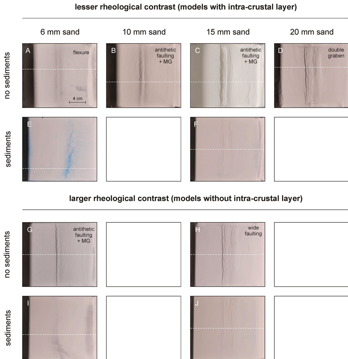
Fig. 3. Map view summary of final reference model structures as a function of brittle layer thickness, the presence of a thin intra-crustal layer and sedimentation. Lighting from the left. MG: marginal graben.
