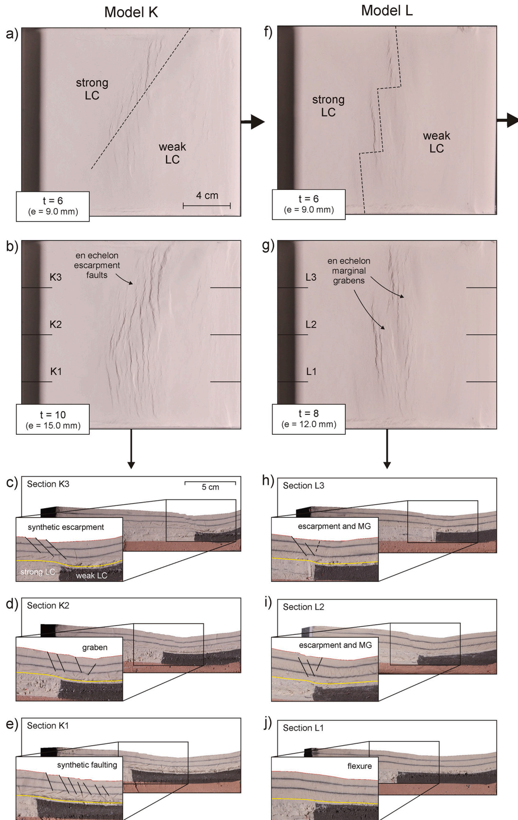
Fig. 8. Surface evolution and cross-sections of series 2 models K and L, aiming to simulate the tectonic setting along the Western Afar Margin during its first and second development phase, respectively (Fig. 1c, d). In map view, dotted lines indicate the transition from a strong LC (lower crust) to a weak lower crust analogue. In section view, the strong and weak lower crustal analogues are light grey and black, respectively. MG: marginal graben.
