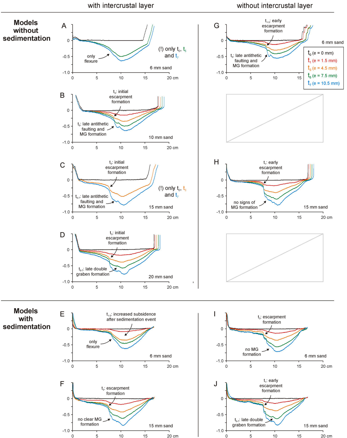
Fig. 6. Subsidence evolution overview of selected experiments from series 1. The graphs, showing cumulative subsidence along a profile through the center of the experiments, are derived from DEMs obtained via photogrammetry techniques. Time steps shown: t_0 , t_1 , t_3 , t_5 and t_7 (i.e. 0, 1.5, 4.5, 7.5 and 10.5 mm or extension, see legend in model G). Note that some time steps are missing in Models A and C. MG: marginal graben.
