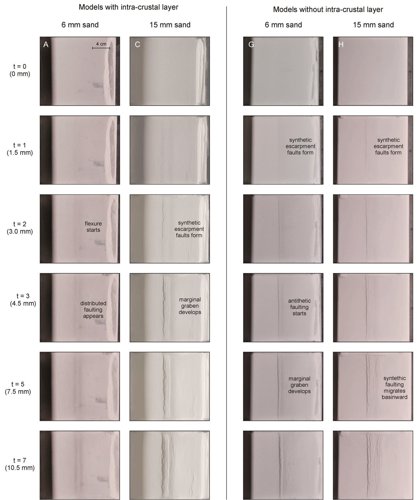
Fig. 5. Comparing surface evolution of selected series 1 models with and without intra-crustal layer. All models are without syn-rift sedimentation.
