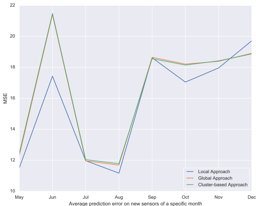
Figure 6: Average prediction error on new sensors of a specific month. The result is obtained by averaging the performance of all the prediction models available for a specific test month.
