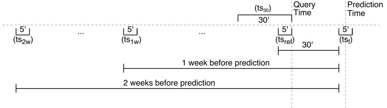
Figure 2: Diagram illustrating time-slot related features.
