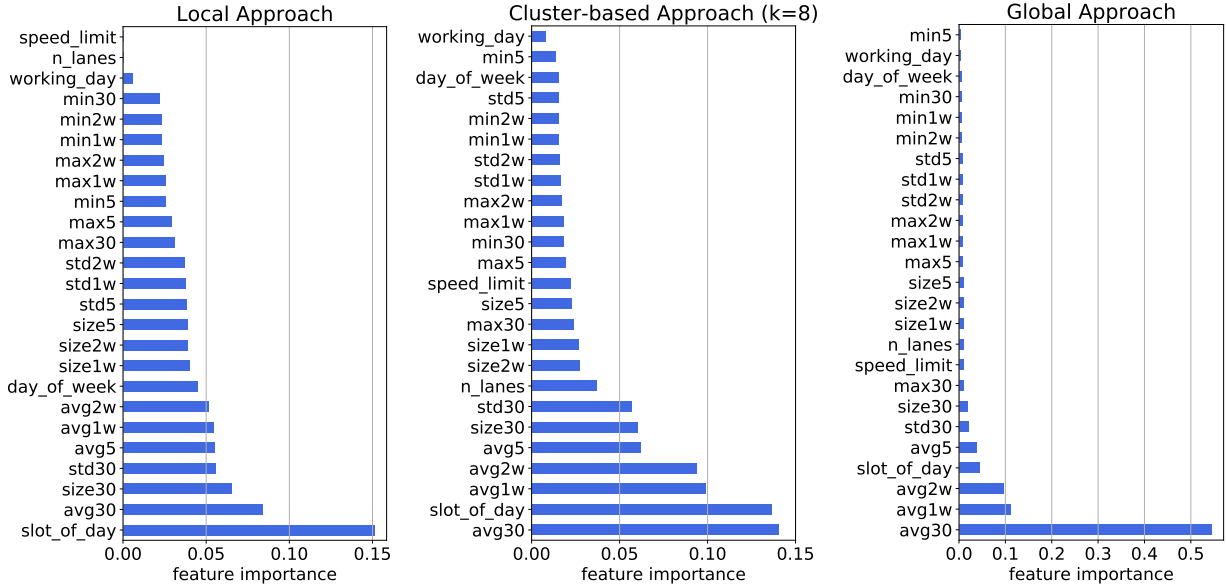
Figure 4: Analysis on the relevance of features. Left-hand side : feature relevance with the local approach. Center side : feature relevance with the cluster-based approach for k=8 . Right-hand side : feature relevance with the global approach.
