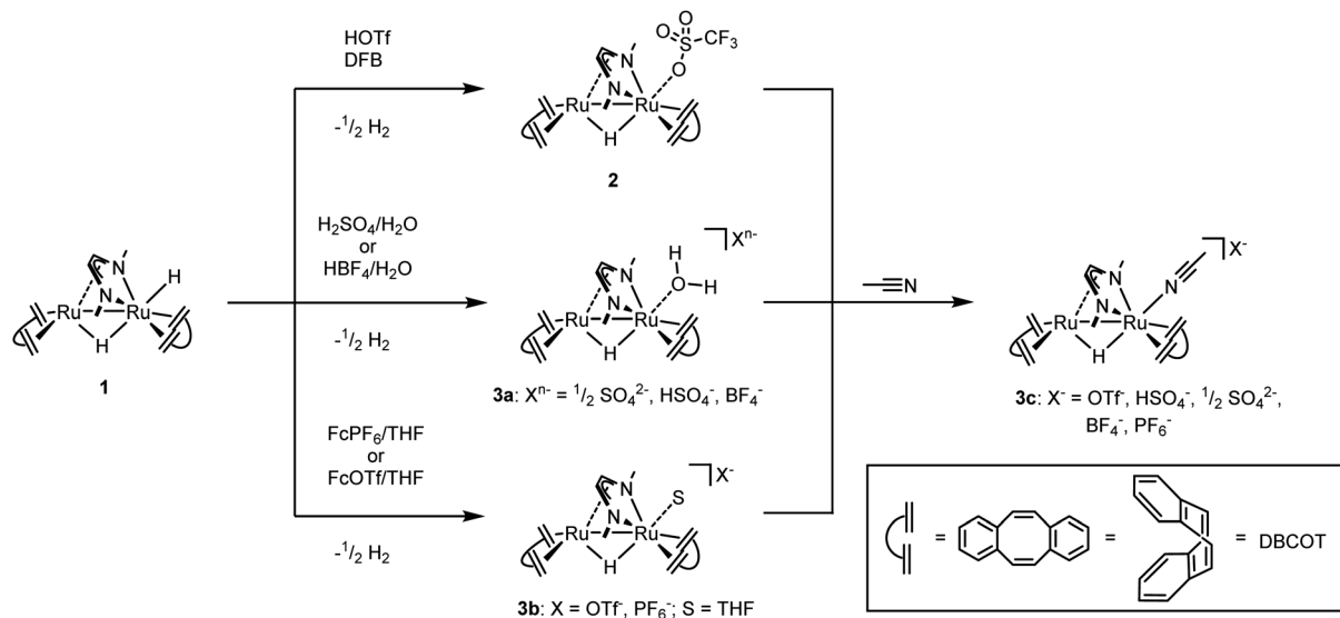
Scheme 1 Syntheses of complexes 2 , 3a , 3b , and 3c starting from 1 . \text{OTf}^- = \text{SO}_3\text{CF}_3^- , \text{Fc}^+ = \text{ferrocenium}^+ , \text{DFB} = 1,2\text{-difluorobenzene} .
