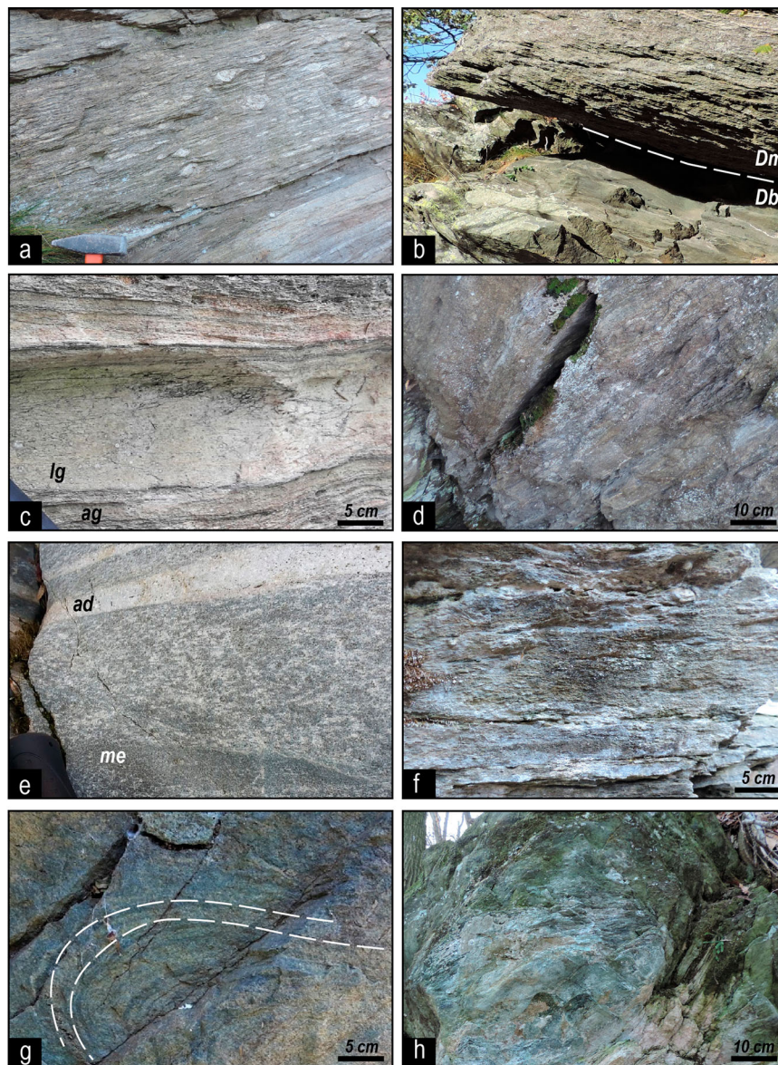
Figure 2. Field images of different lithologies exposed in Valmala: (a) mylonitic augen gneiss (Rocca Solei Unit, N of Vacot, 44^{\circ}33'33'' , 7^{\circ}21'22'' ); (b) stratigraphic contact relationships (dashed white line) between the garnet- and chloritoid-bearing mica schist (Dm) and the fine-grained massive metabasite (Db) (Dronero Unit, N of Santuario di Valmala, 44^{\circ}31'7'' , 7^{\circ}20'31'' ); (c) layer of leucogneiss (lg) interbedded in micro-augen gneiss (ag) (Dronero Unit, S of Chiot del Bosco, 44^{\circ}31'57'' , 7^{\circ}20'46'' ); (d) grayish mica schist with millimeters-thick quartz veins (Valmala Tectonic Unit, Bric Guardia, 44^{\circ}32'50'' , 7^{\circ}19'35'' ); (e) massive meta-quartzdiorite with centimeters-thick mafic enclave (me) and acidic dyke (ad) (Valmala Tectonic Unit, Comba di Valmala, 44^{\circ}32'54'' , 7^{\circ}20'27'' ); (f) carbonate-rich calcschist (Valmala Tectonic Unit, W of Perotto, 44^{\circ}32'34'' , 7^{\circ}20'17'' ); (g) banded metabasite showing the S1 foliation (dashed white lines) deformed by D2 folds (Valmala Tectonic Unit, E of Rora, 44^{\circ}32'56'' , 7^{\circ}20'54'' ); (h) carbonate-bearing serpentinite (Valmala Tectonic Unit, W of Botto, 44^{\circ}32'53'' , 7^{\circ}19'52'' ).
