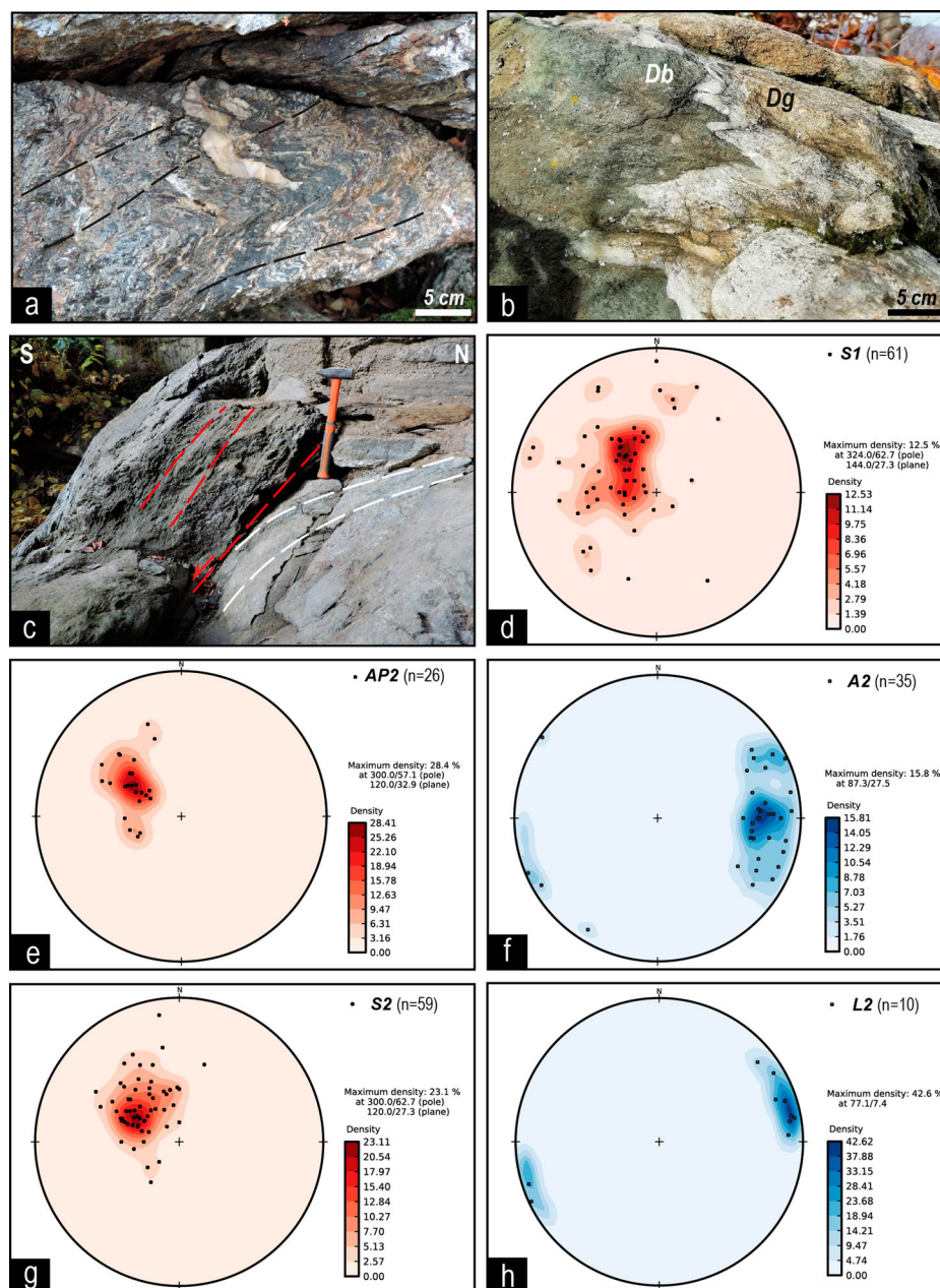
Figure 3. Images of different field-scale structures: (a) D2 crenulation cleavage (dashed black lines) in garnet- and chloritoid-bearing mica schist (Dronero Unit, N of Santuario di Valmala, 44°31'7, 7°20'35); (b) D2 folds deforming the contact between metabasite (Db) and leucogneiss (Dg) (Dronero Unit, E of Santuario di Valmala, 44°30'48, 7°21'2); (c) D3 extensional shear planes (dashed red lines) dragging the S2 foliation (dashed white lines) in mylonitic dioritic gneiss (Valmala Tectonic Unit, Comba di Valmala, 44°32'48, 7°20'30). (d–h) Equal-area lower-hemisphere stereographic projections of different structures (n: number of data; counting method: Fisher distribution): (d) poles of S1 foliation; (e) poles of D2 axial plane (AP2); (f) D2 axes (A2); (g) poles of S2 foliation; (h) D2 stretching lineations (L2).
