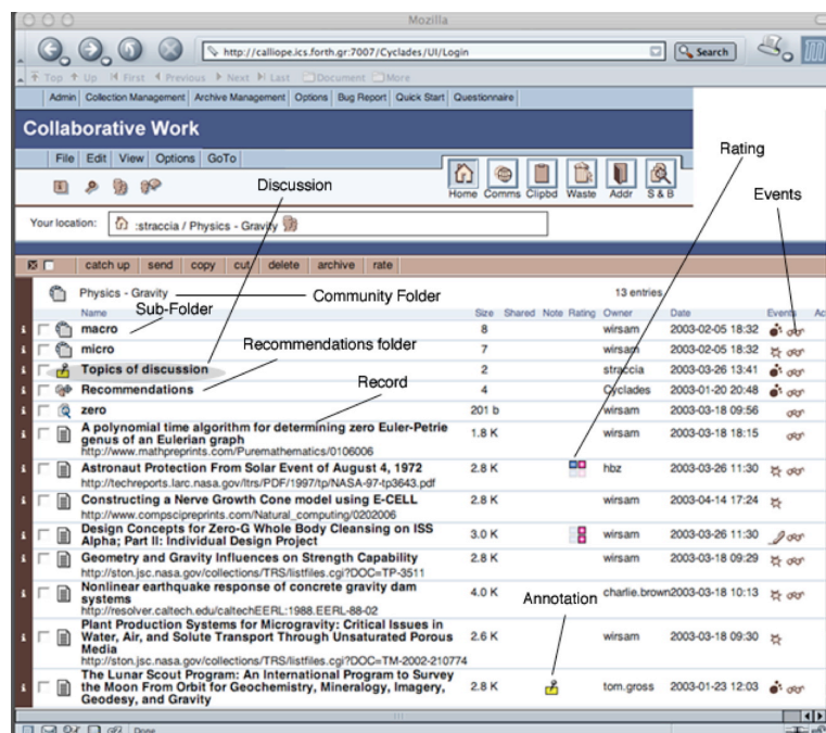
Figure 5. User interface: folder content.
