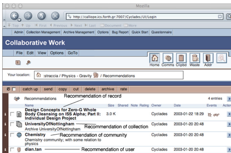
Figure 8. User interface: folder content and recommendations.
