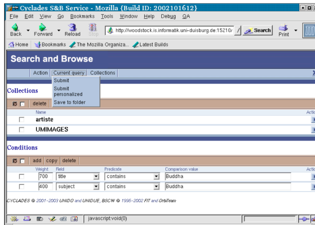
Figure 6. User interface: search metadata records.
