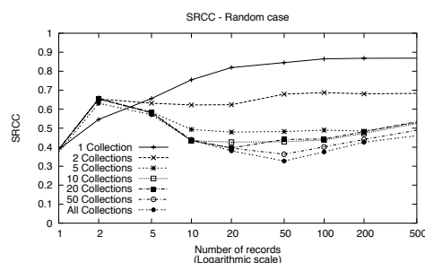
Figure 20. Random case: SRCC values.
