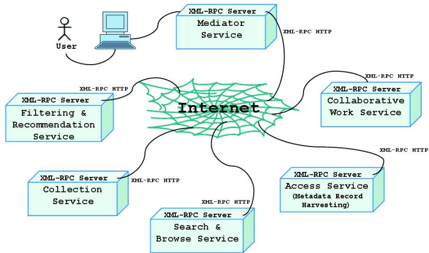
Figure 2. CYCLADES Architecture.
