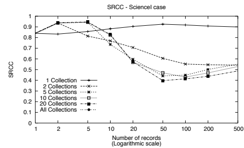
Figure 16. ScienceI case: SRCC values.
