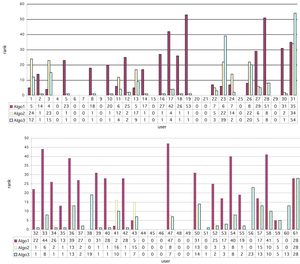
Figure 14. Rank position of correctly recommended users.
