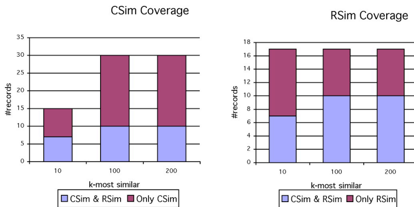
Figure 13. Record recommendation: RSim vs. CSim .
