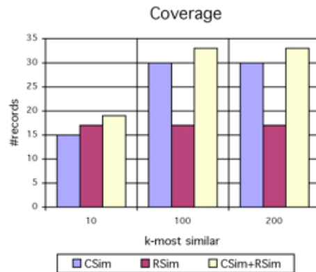
Figure 12. Record recommendation: coverage.
