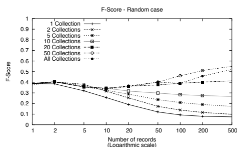
Figure 19. Random case: F-Score values.
