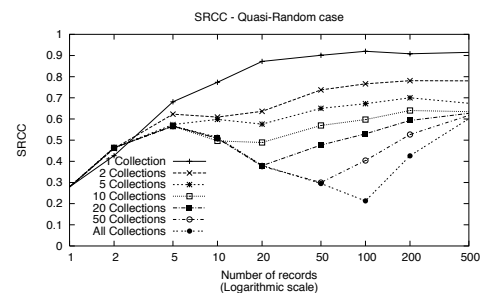
Figure 18. Quasi-random case: SRCC values.
