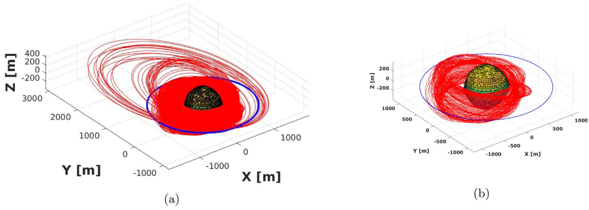
Figure 9. Left panel: full trajectory of the longest-living particle. Right panel: detail of the final orbits from the left panel. The blue circle represents the orbit of Dimorphos around Didymos.
