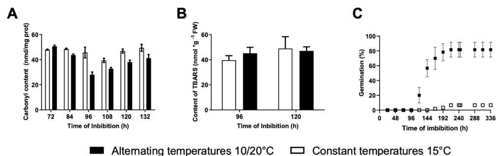
Figure 3. Protein and lipid peroxidation in wild cardoon ( C. cardunculus var. sylvestris ) embryos imbibed at constant ( 15^\circ C ) (open bars) or alternating temperatures ( 20/10^\circ C ) (filled bars). (A) Protein carbonyl content during imbibition of achenes. (B) Lipid peroxidation was measured as TBARS content. (C) Germination dynamics at alternating (circles) and constant temperatures (squares).
