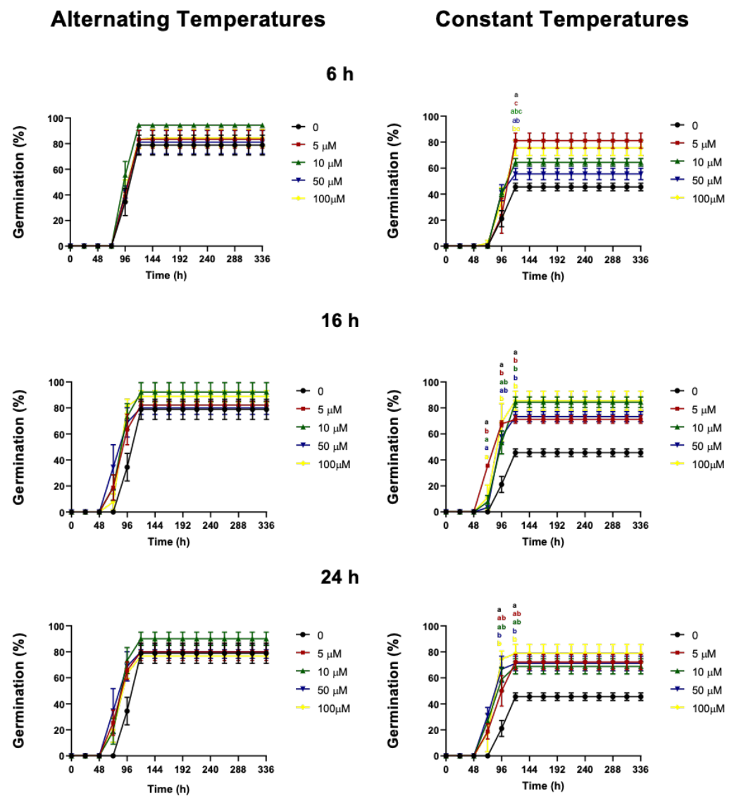
Figure 1. Effects of cyanide on wild cardoon ( C. cardunculus var. sylvestris ) achene germination. Pre-treatments with KCN at different concentrations (5, 10, 50 or 100 \mu\text{M} ) were carried out for 6, 16 or 24 h and then the achenes were imbibed at alternating (10/20 ^{\circ}\text{C} ) or constant (15 ^{\circ}\text{C} ) temperatures. For control treatment (0), achenes were imbibed in water. Different coloured letters represent the significant differences according to one-way ANOVA and Tukey test ( p < 0.05 ) between cyanide-pre-treated samples (KCN) and the control ( \text{H}_2\text{O} ). For alternating temperatures, there was no significant difference.
