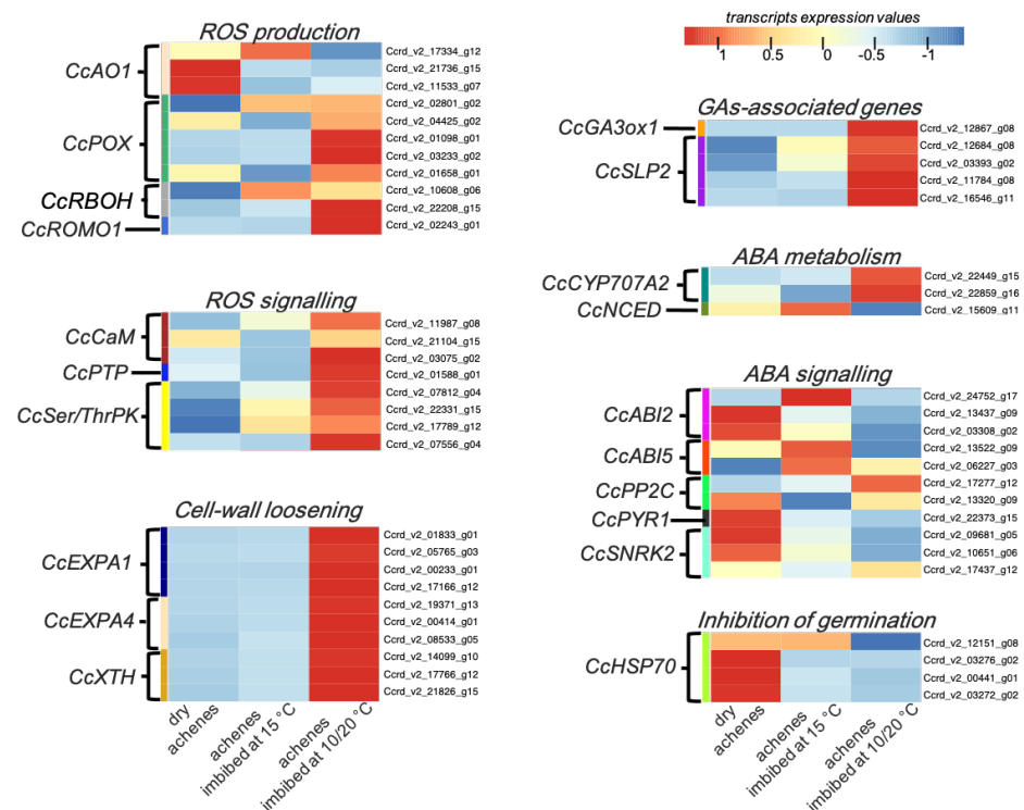
Figure 4. Heat map of ROS signalling, ROS production and seed germination control-associated transcripts in dry, imbibed at constant (15 °C) and imbibed at alternating temperatures (10/20 °C) wild cardoon ( C. cardunculus var. sylvestris ) achenes for 48h. The colour scale represents the log 2 -transformed TPM value.
