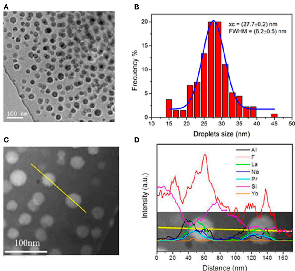
FIGURE 4 | (A) TEM image of the 0.1–0.5 Pr–Yb glass showing phase separation droplets. (B) Droplet size distribution. (C) STEM image of the glass sample where the yellow line is the scanning line along which EDXS analysis was performed (D) .
