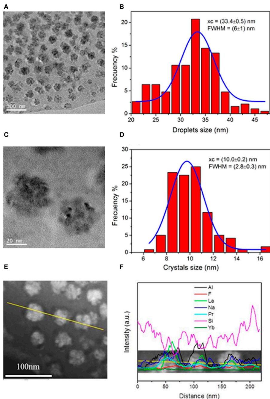
FIGURE 5 | (A) TEM image of the glass-ceramic 0.1–0.5 Pr–Yb 620°C, 20 h and corresponding droplet size distribution (B) . (C) TEM image of two droplets and crystals size distribution inside the droplet (D) . (E) STEM image of the sample and EDXS analysis along the yellow line containing one droplet (F) .
