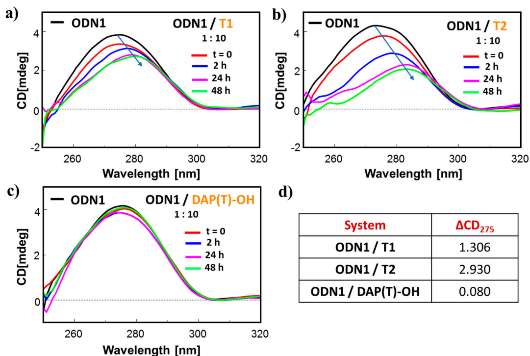
Figure 4. Overlapped circular dichroism (CD) spectra of oligonucleotide 1 (ODN1) (2 \mu M concentration), in the absence (black lines) and presence of T1 (a), T2 (b), and DAP(T)-OH (c) (20 \mu M each) at different times (0, 2, 24, 48 h) after the addition of the target molecules. (d) Differences in the CD signal at 275 nm between the CD spectra of ODN1 before and after 48 h incubation with each added compound. The experiments were carried out in 100 mM KCl, 7 mM Na 2 HPO 4 /NaH 2 PO 4 , pH = 7.2, at 20 °C (optical path = 1 cm).
