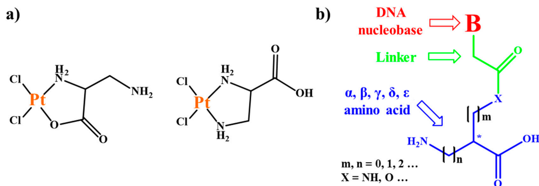
Figure 1. (a) Platinum complexes of L-2,3-diaminopropanoic acid (DAP-OH); (b) general structure of a nucleoamino acid.
