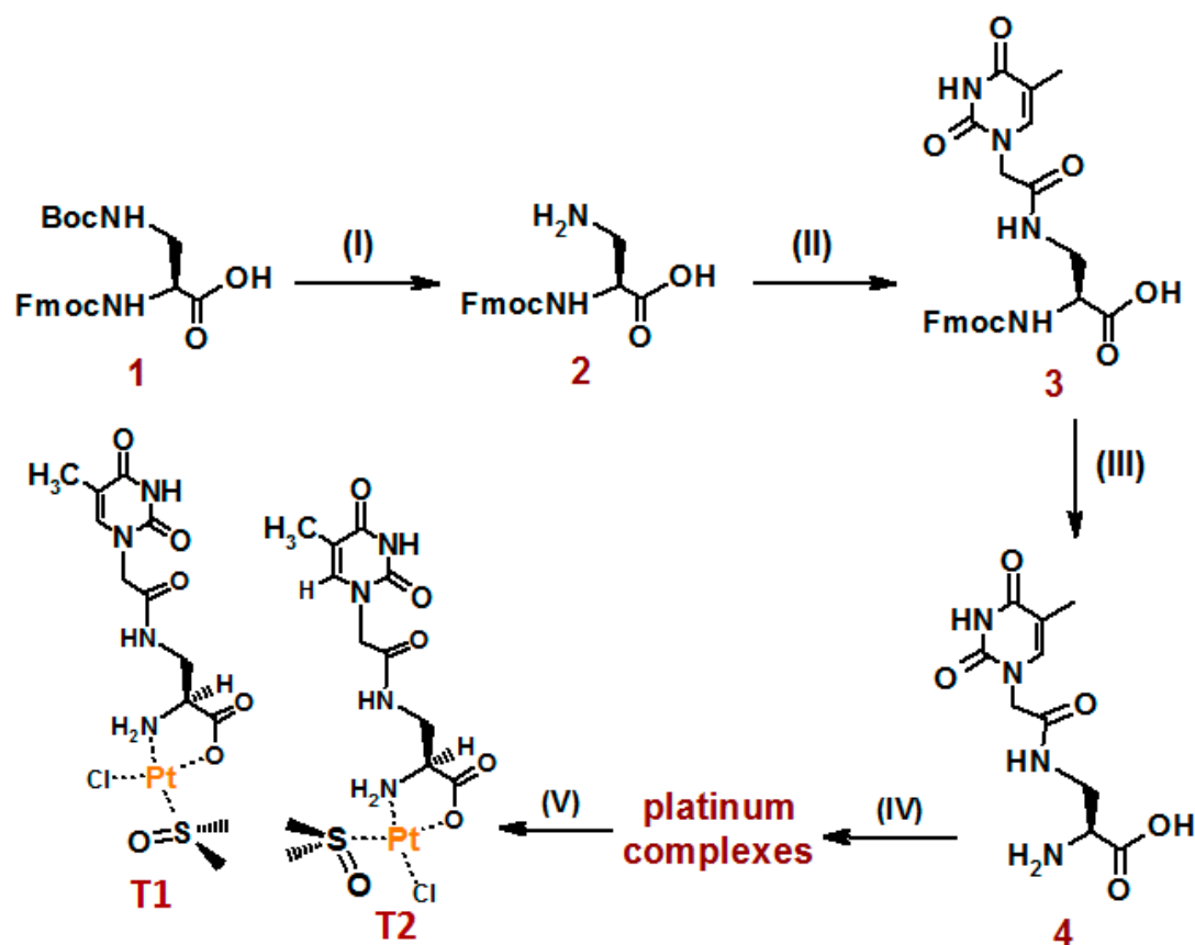
Scheme 1. Synthetic procedure for the preparation of the nucleoamino acid DAP(T)-OH(4) and its platinum complexes. Reagents and conditions: (I) trifluoroacetic acid (TFA)/CH 2 Cl 2 (1:1, v/v ), 45 °C, 1.5 h (98% yield); (II) thymine acetic acid, 1-[bis(dimethylamino)methylene]-1H-1,2,3-triazolo[4,5- b ]pyridinium 3-oxid hexafluorophosphate/ N,N -diisopropylethylamine (HATU/DIEA) in N,N -dimethylformamide (DMF), 2 h, room temperature (r.t.) (80%); (III) piperidine (8 equiv.) in DMF/CH 3 OH (9:1, v/v ), r.t., 10 min (98%); (IV) K 2 PtCl 4 in CH 3 OH/H 2 O (9:1, v/v ), 6 h, r.t., in the dark; (V) dimethyl sulfoxide (DMSO) dissolution of the platinum complexes obtained under conditions IV to favour DMSO-exchange reaction.
