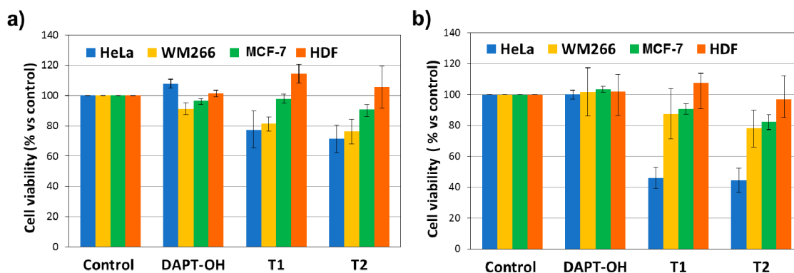
Figure 3. Cell viability assay on human cervical adenocarcinoma (HeLa), metastatic melanoma (WM266), breast adenocarcinoma (MCF-7), and human fibroblasts (HDF). Cells were incubated with T1, T2, or DAP(T)–OH at 25 (a) or 50 (b) \mu\text{M} concentration at 37 °C for 48 h. Cell viability was measured by using the 3-(4,5-dimethylthiazol-2-yl)-2,5-diphenyltetrazolium bromide (MTT) assay. The results are presented as the percentage of living cells with respect to the control (vehicle-treated cells) and are expressed as means \pm SE of at least three independent experiments performed in triplicate.
