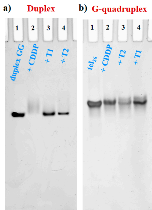
Figure 6. Representative 25% polyacrylamide gel electrophoresis (PAGE) under native conditions relative to the GG-duplex (a) and the G-quadruplex (b) DNA systems (2 \mu M concentration), alone (lanes 1) or incubated for 48 h with 10 equiv. of CDDP, T1 and T2 in 100 mM KCl, 7 mM Na 2 HPO 4 /NaH 2 PO 4 , pH = 7.2. Gel was run at 80 V, at r.t. for 3.3 h in TBE 1 \times buffer.
