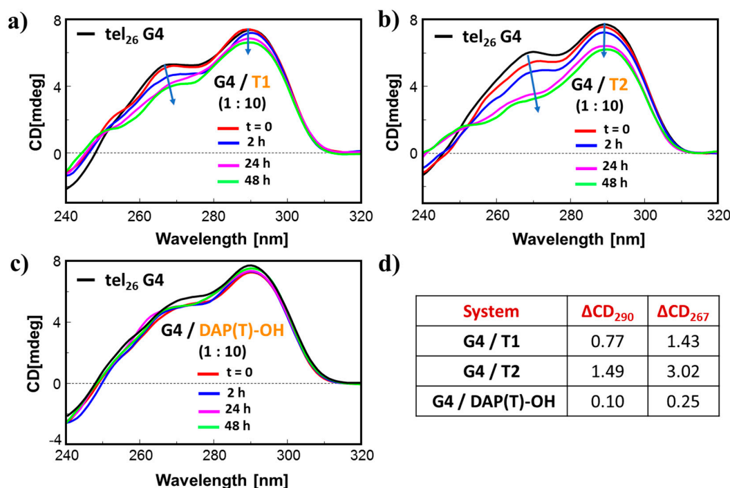
Figure 5. Overlapped CD spectra of the G-quadruplex (G4) tel 26 (2 μM concentration), in the absence (black lines) and presence of T1 (a), T2 (b), and DAP(T)-OH (c) (20 μM each) at different times (0, 2, 24, 48 h) after the addition of the target molecules. (d) Differences in the CD signal at 290 and 267 nm between the CD spectra of the G4, before and after 48 h incubation with each added compound. The experiments were carried out in 100 mM KCl, 7 mM Na 2 HPO 4 /NaH 2 PO 4 , pH = 7.2, at 20 °C (optical path = 1 cm).
