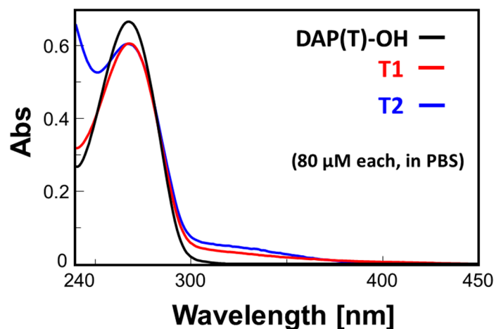
Figure 2. Overlapped ultraviolet-visible (UV-vis) spectra of the two platinum complexes ( T1 and T2 ) and the starting ligand DAP(T)-OH dissolved at 80 \mu M concentration in phosphate-buffered saline (PBS).
