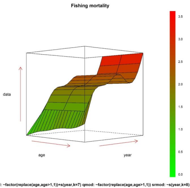
Figure 6.7.3.6. Deep-water rose shrimp stocks in GSAs 17-19. 3D contour plot of estimated fishing mortality at age and year.
