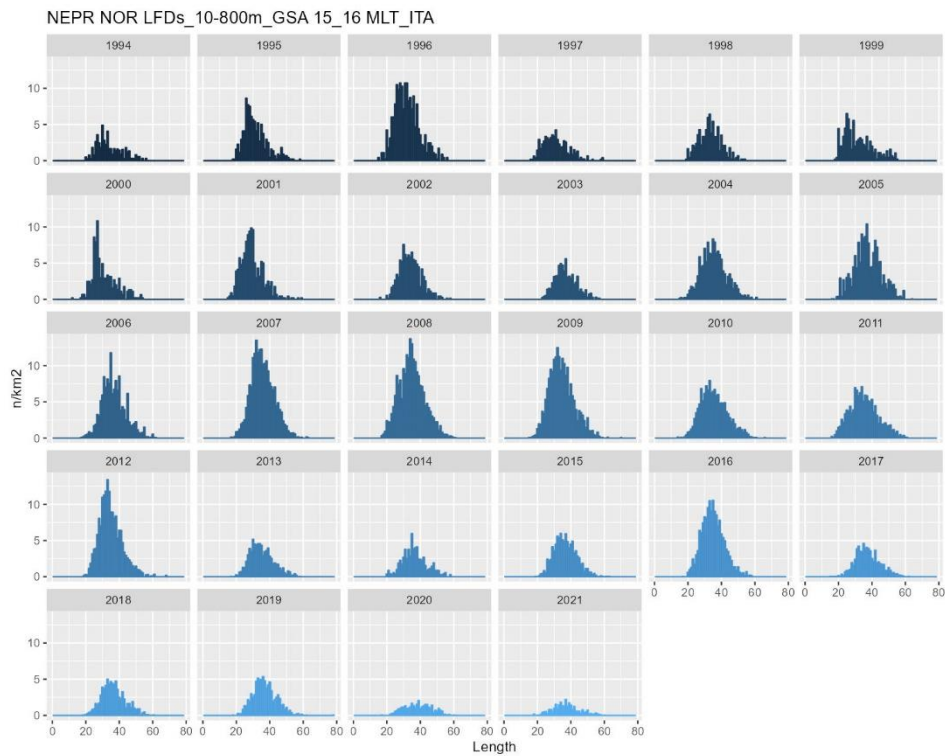
Figure 6.11.2.3.6. Norway lobster in GSAs 15 and 16. Length frequency distribution by year for sexes combined of MEDITS survey.
