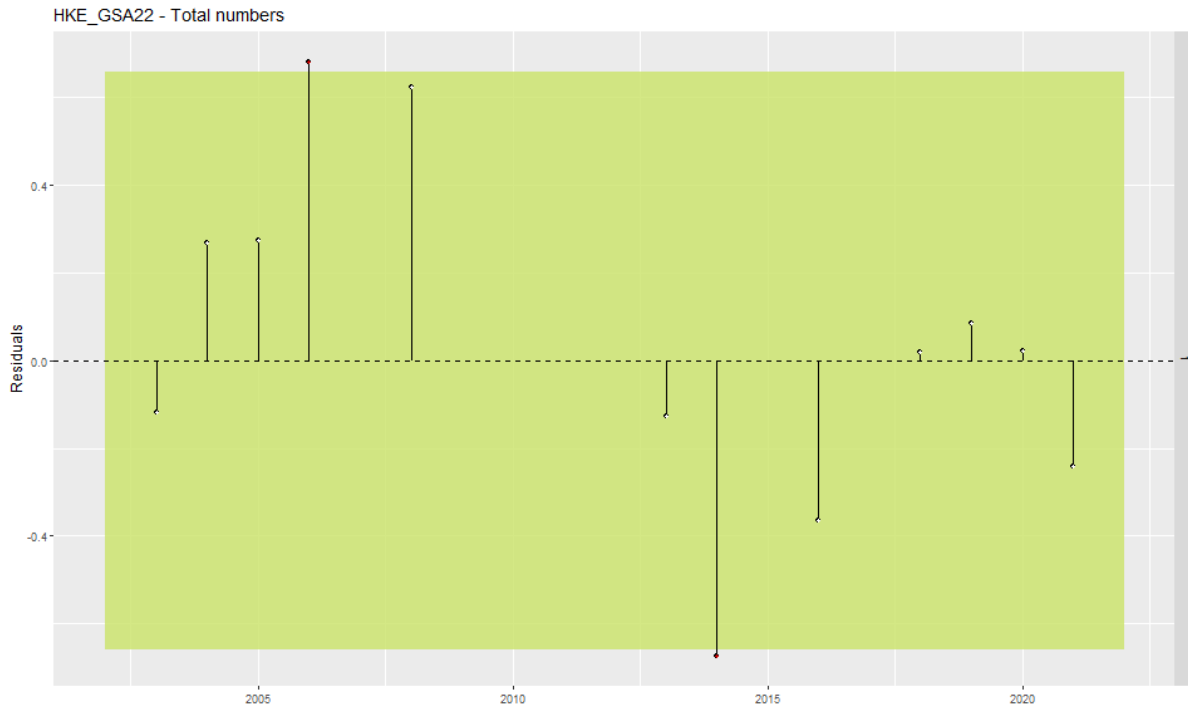
Figure 6.15.3.15. Hake in GSA 22. Residuals of total numbers.
