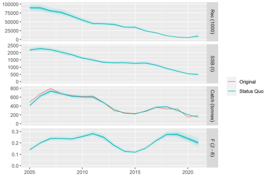
Figure 6.11.3.9. Norway lobster in GSAs 15 and 16. Simulations over summary results.
