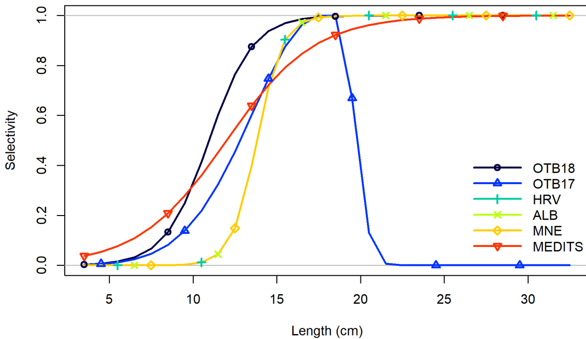
Figure 6.3.3.4 Selectivity by fleet in SS3 run 9. MEDITS selectivity is referred to the years until 2012.
