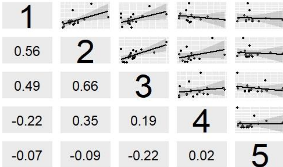
Figure 6.8.3.4. Giant red shrimp in GSA 18-20. Catch internal consistency plot
