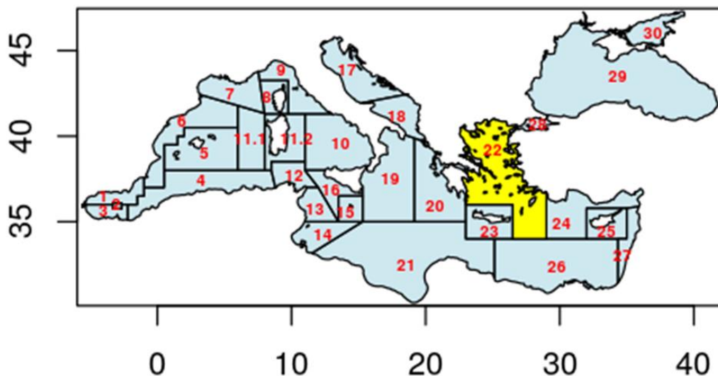
Figure 6.15.1.1. Geographical location of GSA 22.
