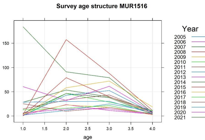
Figure 6.12.27 – Striped red mullet in GSA15_16: Index at age numbers (*1000) used in the assessment (age0 and age5+ removed).
