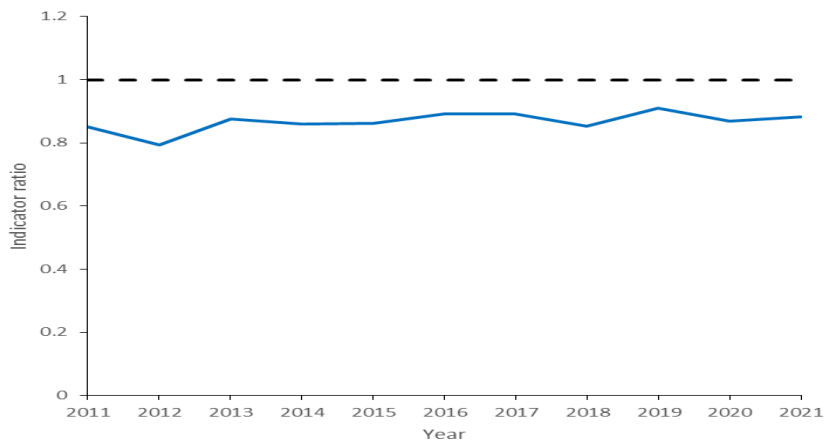
Figure 5.3.2 Red mullet in GSAs 17 and 18: Length indicator (mean length of fish in the catch divided by MSY proxy reference length). The exploitation status is below F_{MSY} proxy when the indicator ratio value is higher than 1 (shown by the dashed line).
