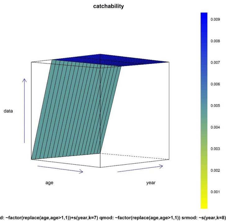
Figure 6.7.3.7. Deep-water rose shrimp stocks in GSAs 17-19. 3D contour plot of estimated catchability at age and year.
