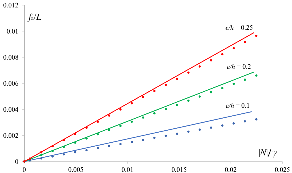
FIGURE 3. Case (a): deflection of a masonry-like cantilever beam f_a/L vs normal force |N|/\gamma for different values of the eccentricity.
