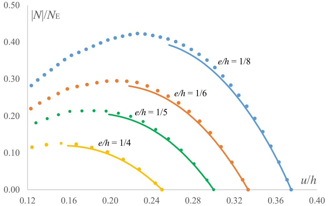
FIGURE 5. Case (a) : ratio |N|/N_E vs ratio u/h for different values of the initial eccentricity e . From the left: e/h = 1/4 , e/h = 1/5 , e/h = 1/6 , e/h = 1/8 .
