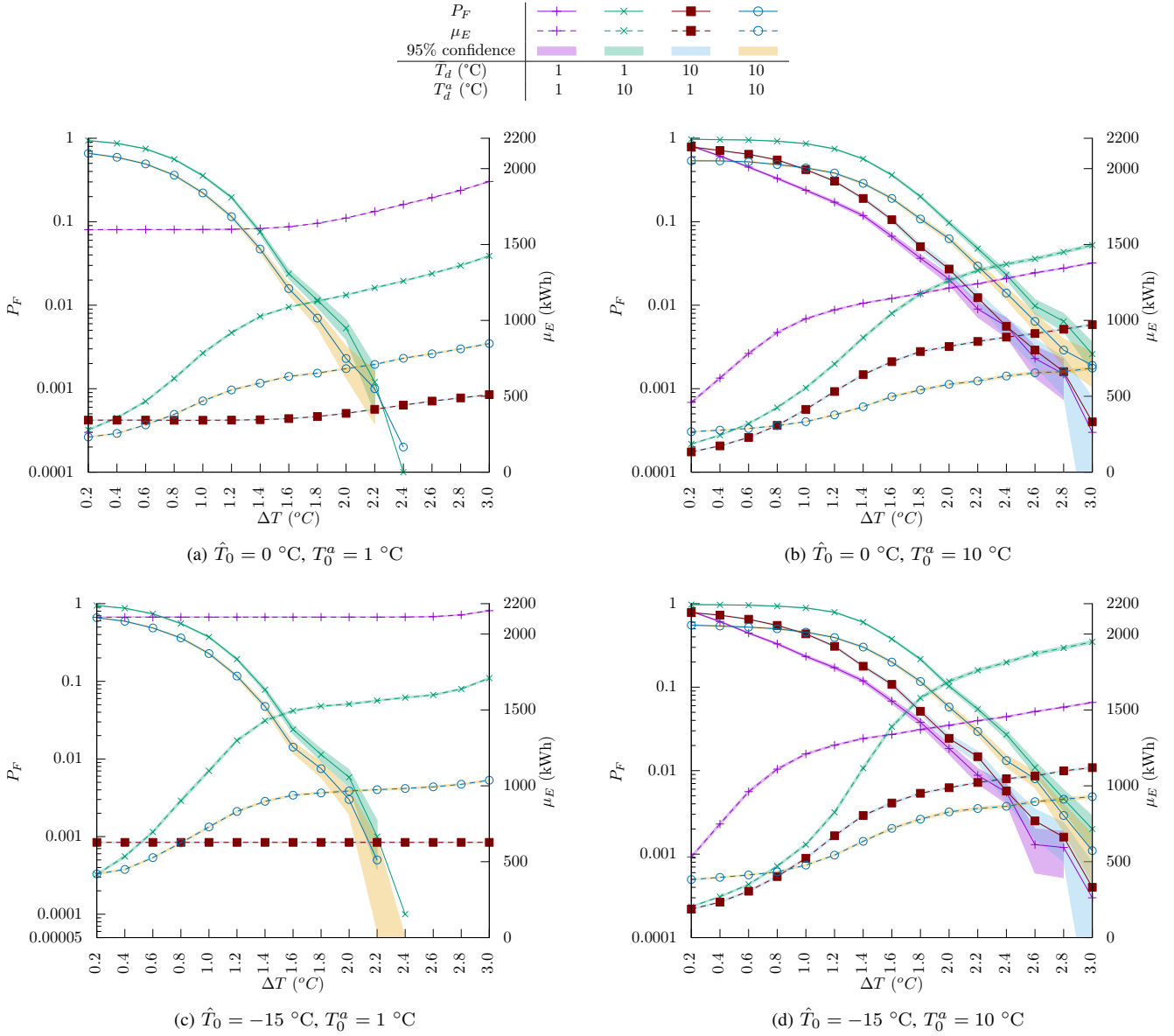
Figure 3. Probability of failure, i.e., freezing, within one day ( P_F , in log scale, continuous lines) vs expected energy consumption ( \mu_E , dashed lines) at increasing of \Delta T , with shaded confidence intervals obtained with a 95% confidence level.
