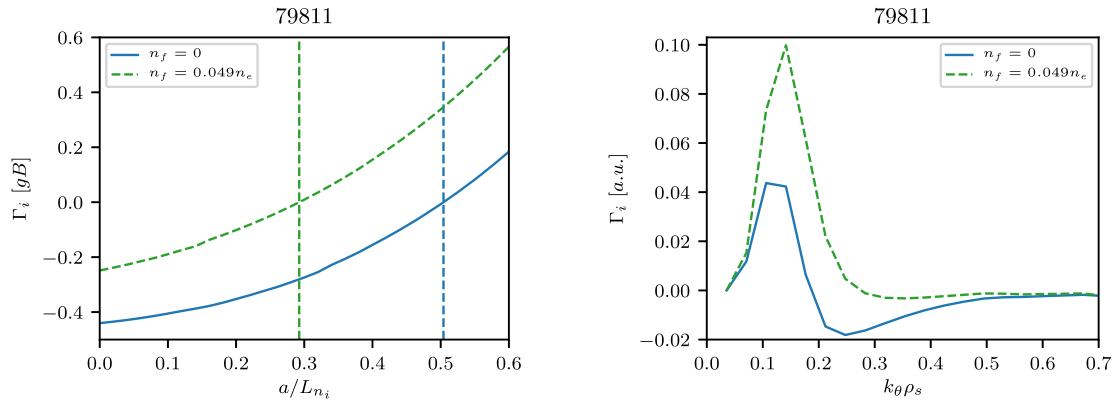
(c) Ion particle flux as a function of ion density gradient. The vertical dashed lines correspond to zero particle flux. (d) Ion particle flux spectrum w/o and including fast ions when a/Ln_i = PF_i w/o fast ions.
