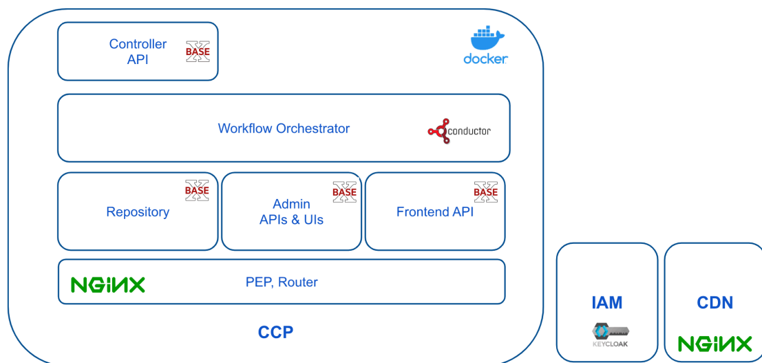
Figure 10: Technological architecture implementation
