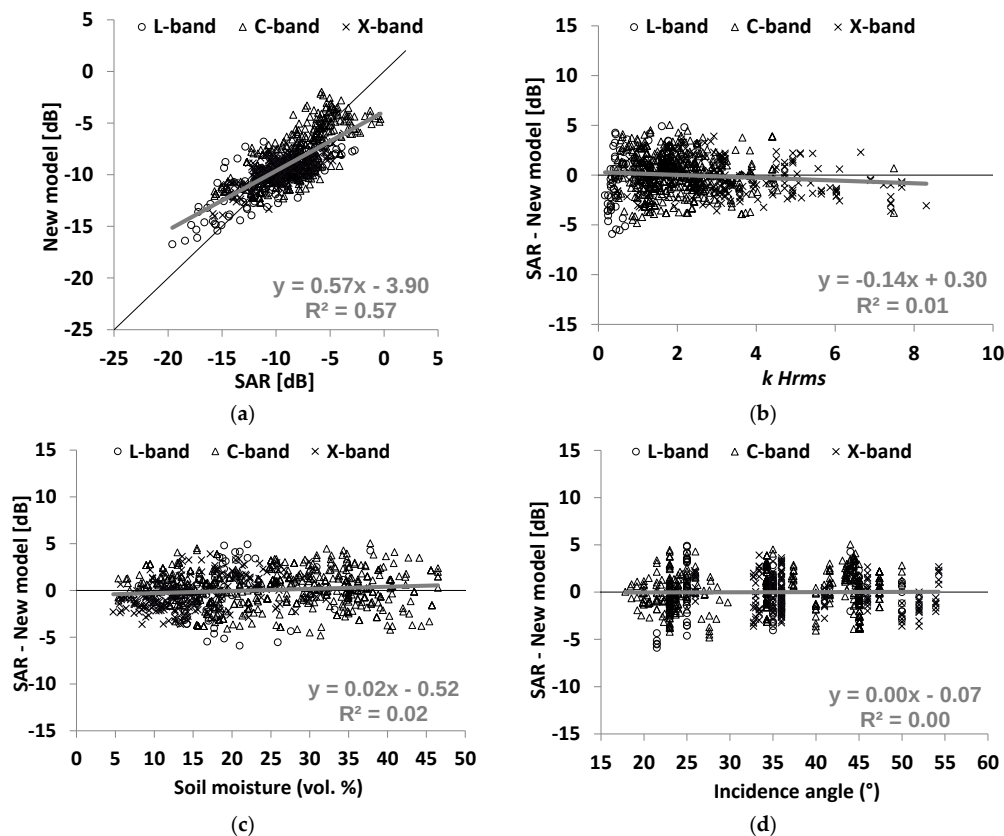
Figure 4. (a) Comparison between \sigma^0 in the new model and \sigma^0 measured (for all SAR bands) for VV polarization; (b) the difference between SAR and the new model as a function of surface roughness ( kHrms ); (c) the difference between SAR and the new model as a function of soil moisture ( mv ); and (d) the difference between SAR and the new model as a function of incidence angle. The best regression model is plotted in gray.
