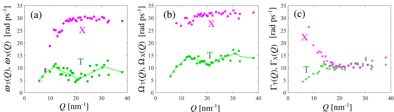
FIG. 4. (a) Q dependence of the frequencies \omega_T (green full circles) and \omega_X (magenta full circles) as obtained from the fits to C_T(Q, t) . The green dotted-dashed spline curve through the T points is just a guide to the eye. (b) Same as panel (a) but for the undamped frequencies \Omega_T (green full squares) and \Omega_X (magenta full squares). (c) Damping coefficients \Gamma_T (green asterisks) and \Gamma_X (magenta asterisks).
