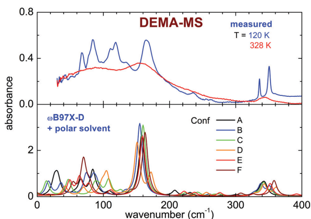
Fig. 7 Far infrared experimental spectra of DEMA-MS measured at the highest and lowest temperature (top) and calculated spectra for different conformers of the ionic couples obtained at the \omega B97X-D/6-31G** level of theory with the inclusion of a polar solvent (bottom).
