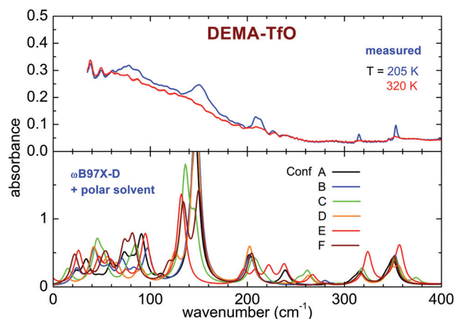
Fig. 8 Far infrared experimental spectra of DEMA-TfO measured at the highest and lowest temperature (top) and calculated spectra for different conformers of the ionic couples obtained at the \omega B97X-D/6-31G** level of theory with the inclusion of a polar solvent (bottom).
