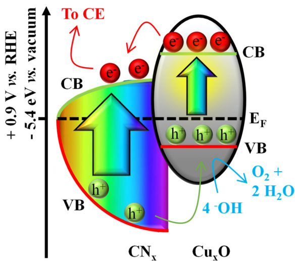
Fig. 11 Approximate band diagram for the \text{CN}_x/\text{Cu}_2\text{O} heterojunction. The positions of VB (valence band) and CB (conduction band) edges for a- \text{CN}_x are represented by red and green curves, respectively. The VB–CB edge separation for \text{CN}_x is proposed considering the E_G values reported in Fig. 2. The Fermi level ( E_F ) position on the vacuum scale was deduced from the work function values reported in Fig. S7.†
