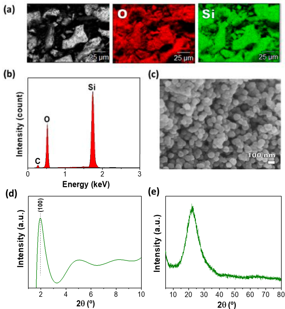
Figure 2. Analysis of SiO 2 obtained from rice husk: (a) EDS chemical mapping, (b) EDS spectrum, (c) SEM-FEG image, (d) XRD at low angle, and (e) XRD at conventional angle.
