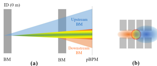
Figure 2: (a) Schematic representation of the radiation contributions from the BMs and the ID. (b) Front view of the pBPM. Central sensors intercept both BM and ID radiation, while peripheral sensors predominantly detect BM radiation, enabling spatial separation of the two components.
