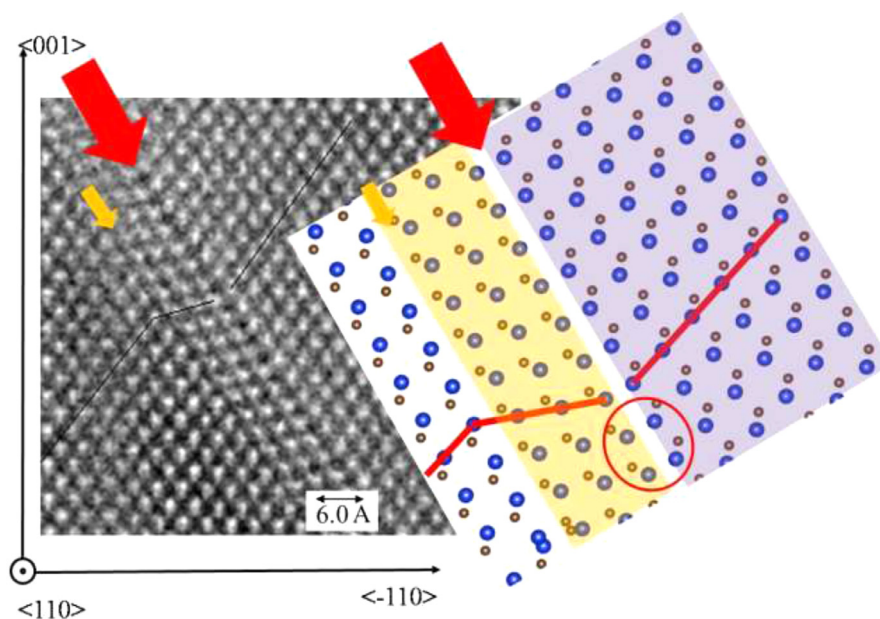
Fig. 8. High-resolution bright-field -STEM image of an IDB laying along the (\bar{1}11) plane and its reconstruction on the right. The yellowish shaded region in the reconstruction represents the SF<math>\langle 3 \rangle</math> associated with the IDB. The red arrow represents the plane of the Si-Si bond while the yellow arrow represents the end of the SF<math>\langle 3 \rangle</math> associated with the IDB. (For interpretation of the references to color in this figure legend, the reader is referred to the web version of this article.)
