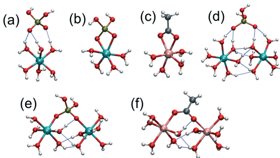
Fig. 5 Optimized structures of hydrated metal ions: single Co ion with a phosphate ligand (a) hydrogen bonding with ligand water molecules and (b) directly coordinating with Co; (c) a single Mn ion with an acetate ligand; no bridge models of two Co ions with a phosphate ligand (d) hydrogen bonding with ligand water molecules and (e) directly coordinating with Co; and (f) no bridge models of two Mn ions with an acetate ligand. All models were calculated with the S_0 state as ground states (red: oxygen, white: hydrogen, yellow: phosphorus, gray: carbon, pink: Mn, and cyan: Co atoms).
