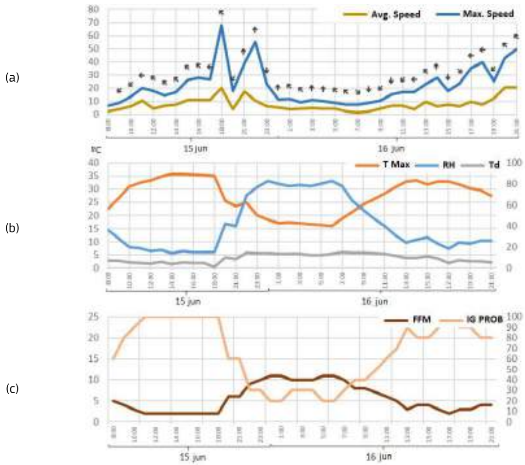
Figure 53. Meteorology station of Villardeciervos – 2775X, at 850 m above sea level. A) Wind speed, B) Temperature and relative humidity, C) Fine Fuel Moisture (FFM) and ignition probability (IG PROB). Sources: AEMet and Castilla y León Forestry Department.
