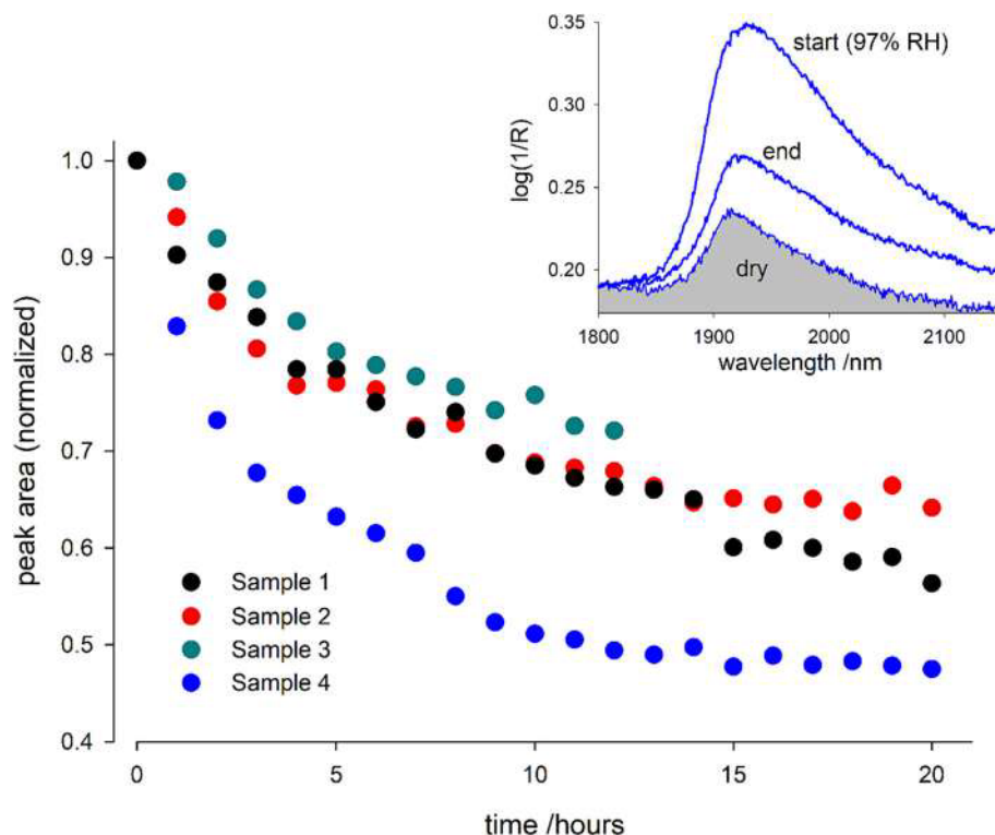
Fig. 7. Water desorption kinetics for the different mortars (see legend) as deduced by NIR reflectance spectroscopy. The inset shows relevant NIR spectra acquired for the mortar specimen 4 at the beginning and at the end of the kinetic experiments (the shaded NIR spectrum refers to the same sample when fully dried).
