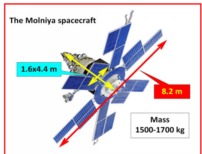
Fig. 2. A sketch of a Molniya spacecraft with its characteristic “daisy” look, as inspired by the six big solar panels. The spacecraft sports a size of 4.4×8.2×8.2 m, with a typical mass about 1500–1700 kg. Note that the two high-gain antennas, symmetrically placed at the two sides of the bus, are not displayed in this figure.
