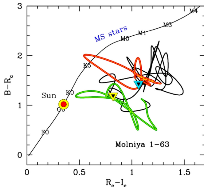
Fig. 8. The observed color path of Molniya 1–63 along its rotation, as from the 2016 Loiano observations (see Fig. 5, right panel) in the (R_c - I_c) vs. (B - R_c) diagram. The lightcurve maxima (that is when solar pads are reflecting) are singled out in green (primary peak) and red (secondary peak), while the black line mainly traces satellite bus reflectance. The big blue and yellow triangles mark respectively the time- and luminosity-averaged colors. For comparison, the (R_c - I_c) vs. (B - R_c) locus for Main-Sequence stars of different spectral type after [15] is also displayed on the plot, marking the Sun's location. .
