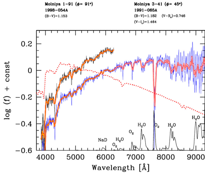
Fig. 7. The reflectance spectra of Molniya 1–91 (black curve) and 3–41 (blue curve), as from BFOSC spectroscopic observations in Loiano. Molniya 1–91 has been observed through grism GR3, while Molniya 3–41 data are from the GR3+GR5 combination ( R \sim 400 ). Both spectra have been smoothed (yellow-dotted moving average on the plots) for better display. The solar spectrum is over-plotted (within arbitrary offset), for comparison (red dotted curve). The absorption features in the satellite spectra are due to the Sun or the telluric absorptions, in the near infrared, mainly by water vapor and Oxygen, as singled out in the lower sketch. Note the fairly “reddish” color of both Molnias, compared to the Sun.
