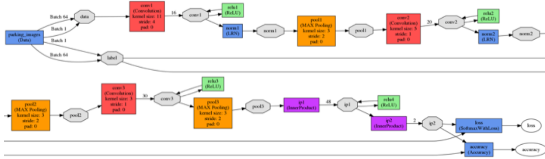
Figure 5 – The neural network used in our solution
