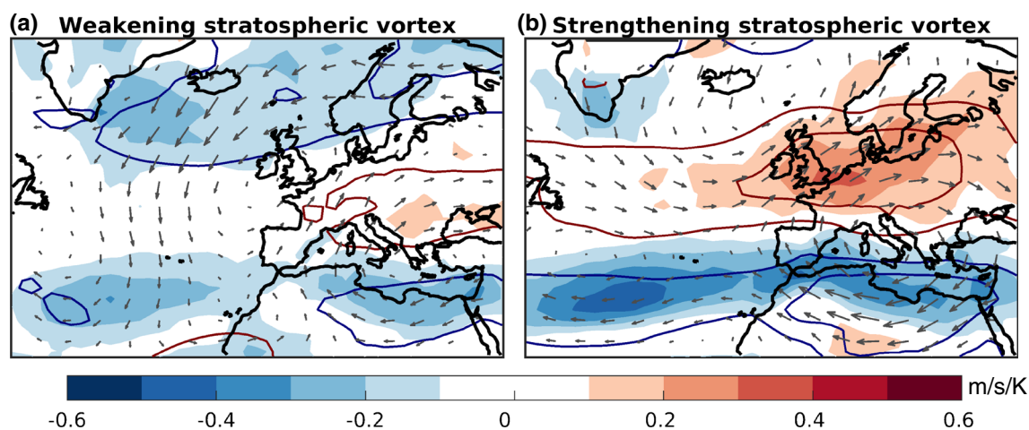
Fig. 2 As in Fig. 1 but for the climate change response in the 98 percentile of the annual distribution of daily wind speed at 850 hPa ( \text{m s}^{-1} \text{K}^{-1} ) conditioned on the response of the stratospheric vortex. Each panel shows the average response for the 6 CMIP5 models with the most negative (a) and most positive (b) change in the vortex strength. The vortex strength is evaluated as the zonal-mean
