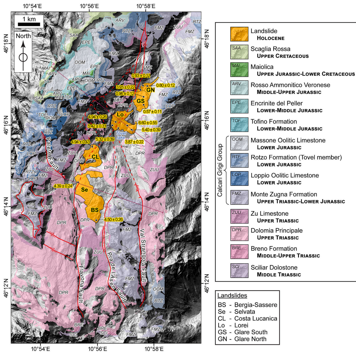
Fig. 3. Geological map of the study area, showing outcropping, major faults, and landslide bodies. Cosmogenic sampling locations are indicated by black dots, and corresponding ^{36}\text{Cl} exposure ages are highlighted in yellow. The traces of the two geological profiles reported in Fig. 5 are shown in purple.
