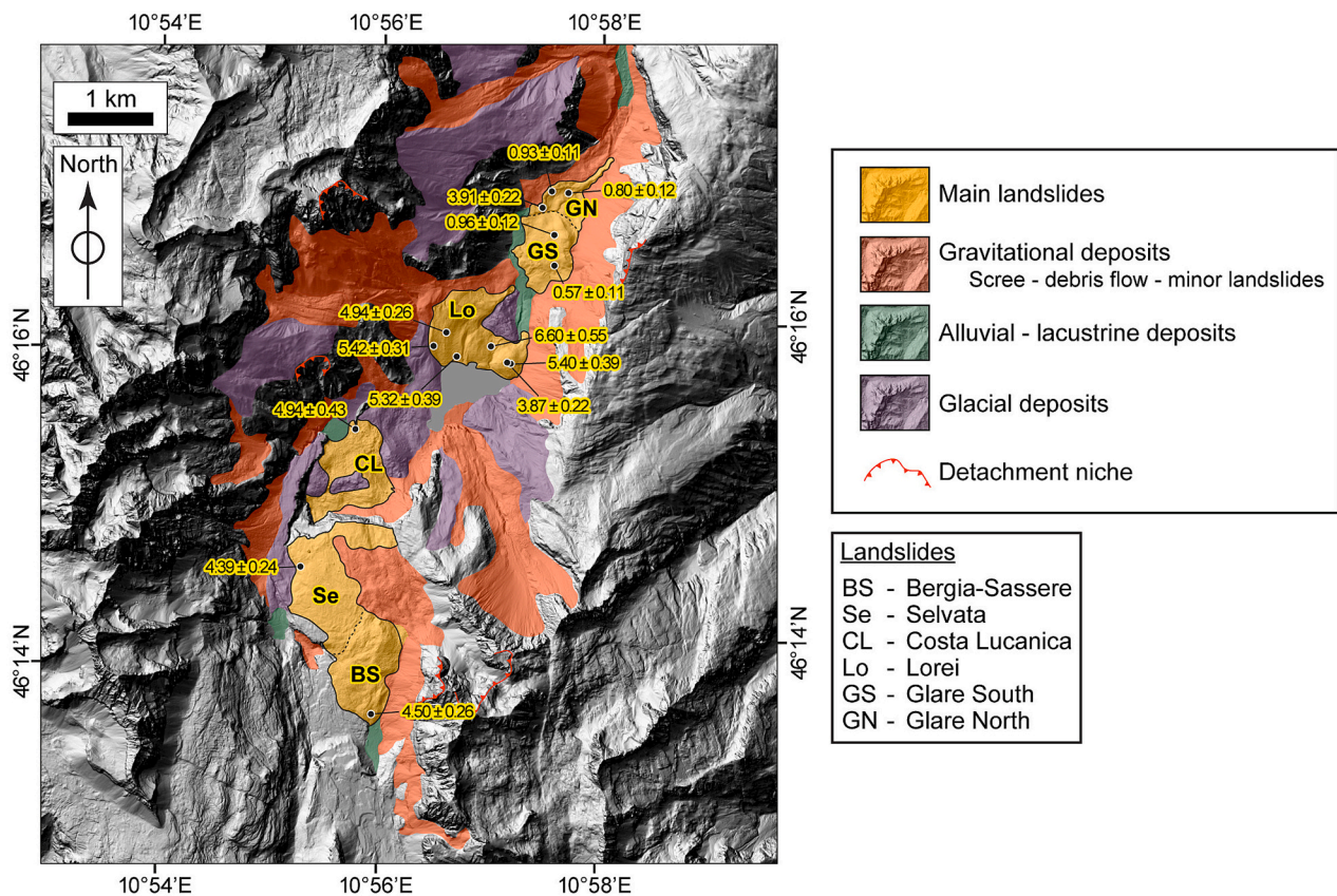
Fig. 6. Map of the central stretch of the Tovel Valley. The main Quaternary deposits are reported, together with the investigated landslide deposits. Cosmogenic sampling locations are indicated by black dots, and corresponding ^{36}\text{Cl} exposure ages are shown for each sampled boulder.
