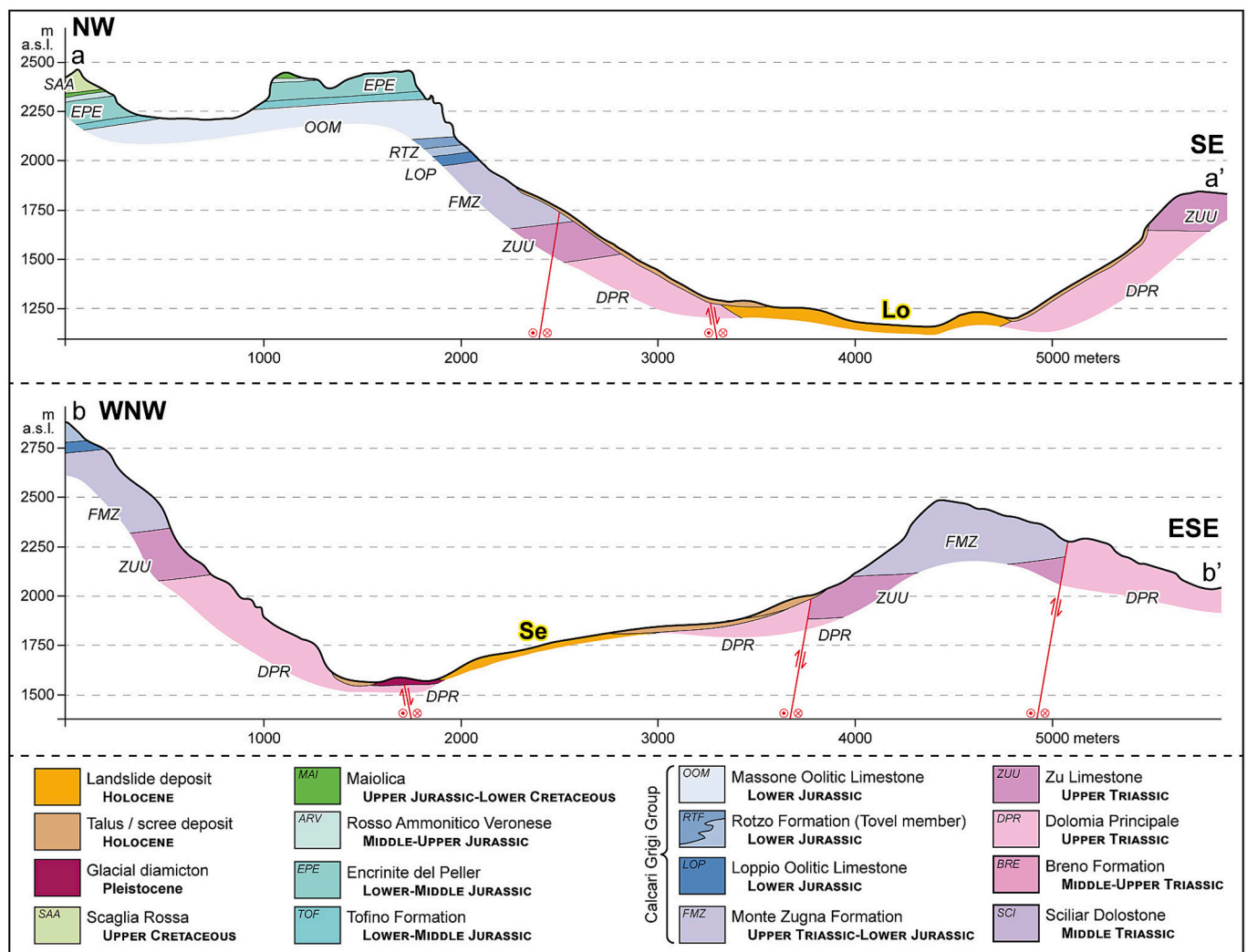
Fig. 5. Geological profiles across the Tovel Valley in the area north of Lake Tovel (a-a') and across the southern plateaux (b-b'). The traces are shown in Fig. 3.
