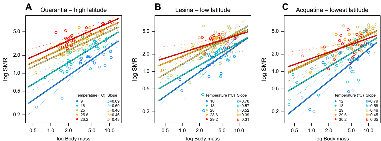
Fig. 2. Standard metabolic rate (SMR; \text{J day}^{-1} ) in relation to dry body mass ( M , mg) across temperature levels at each collection site. (A) Quarantia, high-latitude population; (B) Lesina, low-latitude population; (C) Acquatina, lowest-latitude population. b represents the scaling exponent (slope) of the metabolic rate against body mass for each temperature level.
