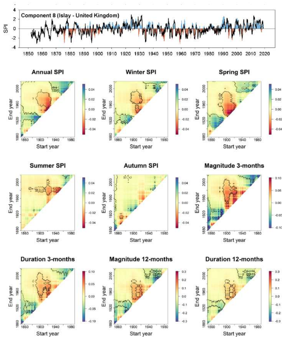
Figure 17: Temporal evolution of the SPI-12 series of component 8 in color and the series of the most representative station (black line). The correlation between the series of the component and the series of the station is r = 0.70 . Also shown are heat maps of 30-year running trends in annual and seasonal SPI and 3- and 12-month SPI drought duration and magnitude for the station of Islay (United Kingdom). X and Y-axes indicate the start and end years, respectively, of the time slices for the running trend analysis. The scale indicates the magnitude of the trend based on the slope of the linear regression analysis. Dotted lines indicate periods with a significant trend ( p < 0.05 ).
